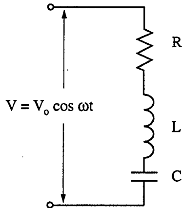
FIGURE 3. Series RLC Circuit With Applied Voltage, V .
