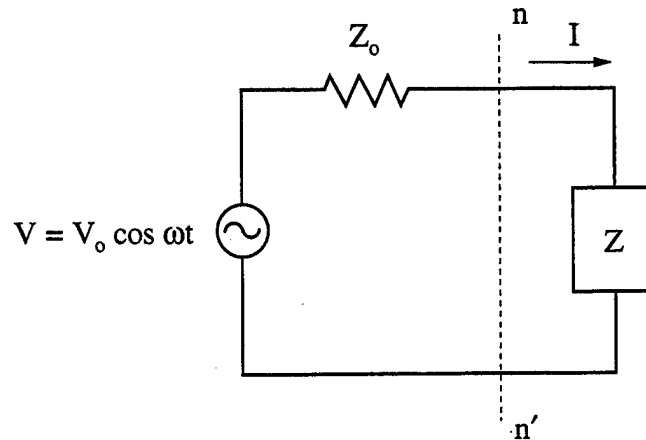
FIGURE E-1. Voltage Generator.
