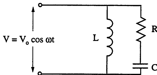
FIGURE 7. Using a Parallel Inductance as a Matching Element for a Hypothetical Series R C Antenna.
