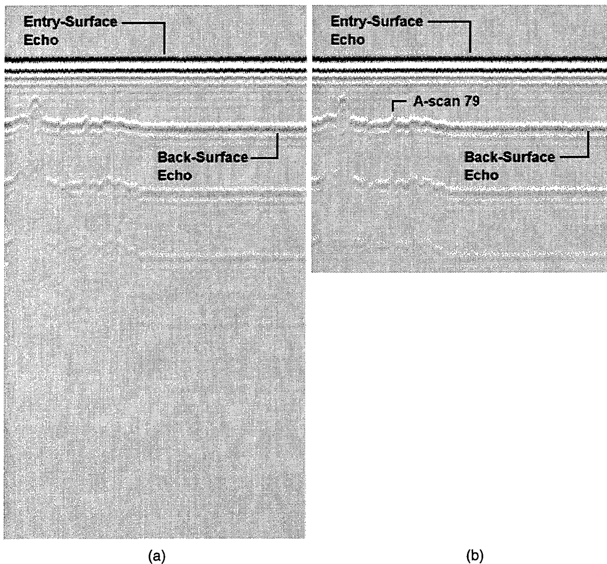
Figure 4 -- B-scan number 89: (a) original, and (b) after eliminating last 256 points from each A-scan.
