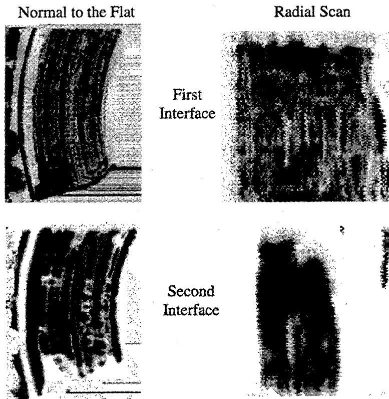
FIGURE 3.4-2 Ultrasonic C-Scan of Failed Rotor Disc, Sample R2C
