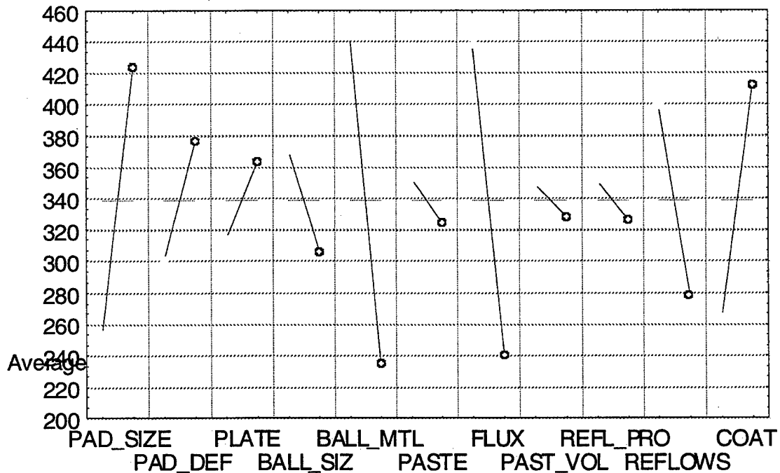
PBGA169 Thermal Cycling Mean Analysis
