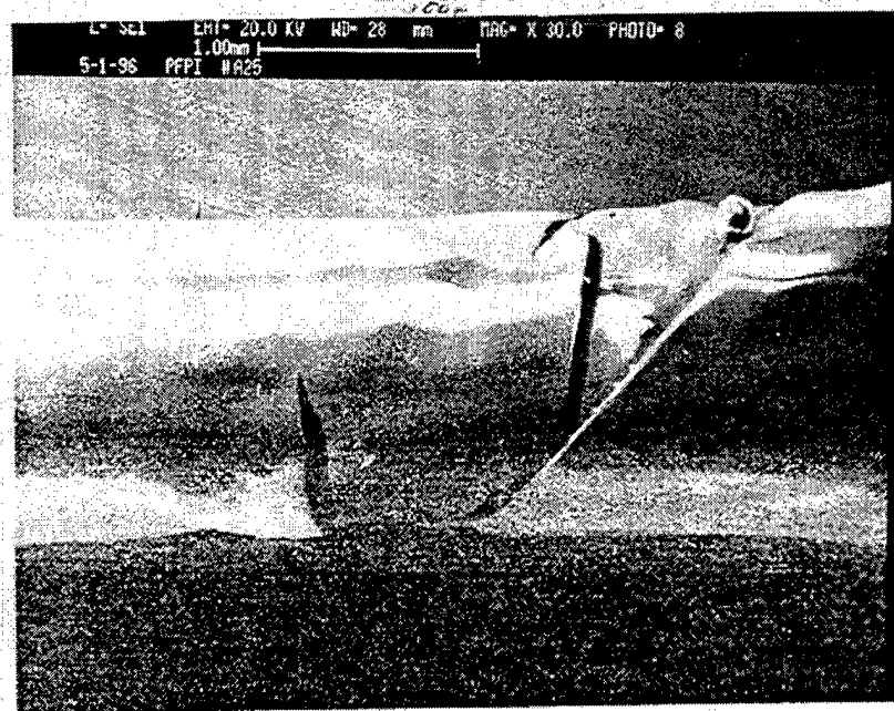
(b) Insulation with Cracks and Adhesive Bead Extruded from Sample B in Table 14
