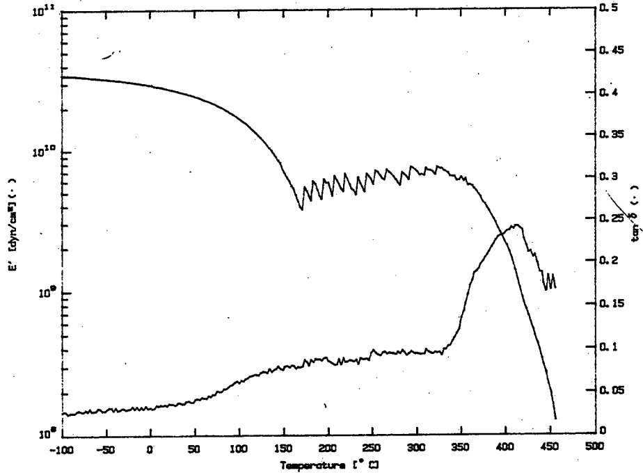
Figure 2. RDA Spectrum of PFPI (4BDAF/PMDA Formulation)
