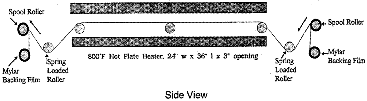
Figure 13. Schematic of Continuous Film Processing Oven
