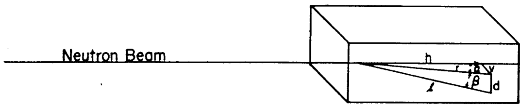
Fig. 7.2 Geometric Relations Involved When Using Plate as Both Radiator and Detector
