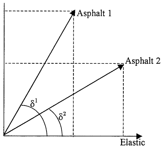
Viscoelastic Viscous vs. Elastic Binder Portion
