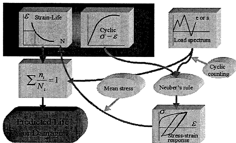
Figure 2: Block diagram for fatigue life prediction model
