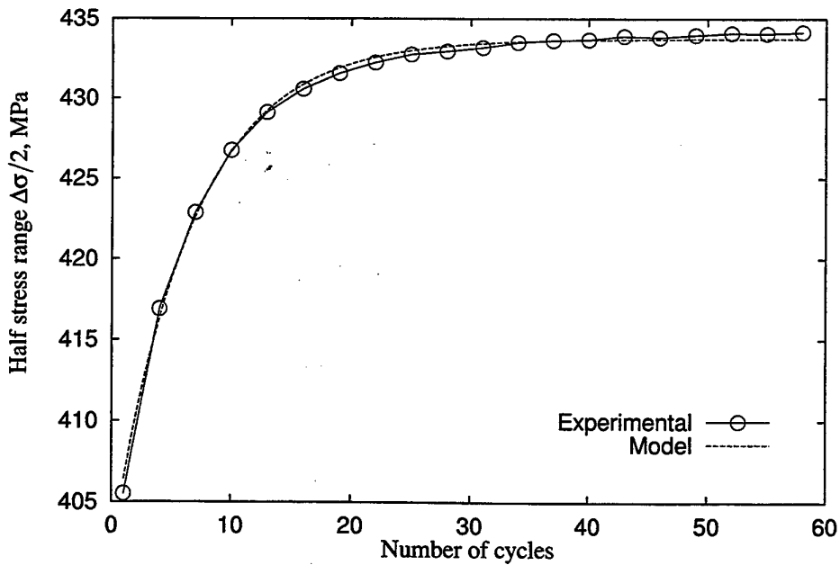
Figure 5: Isotropic hardening curve
