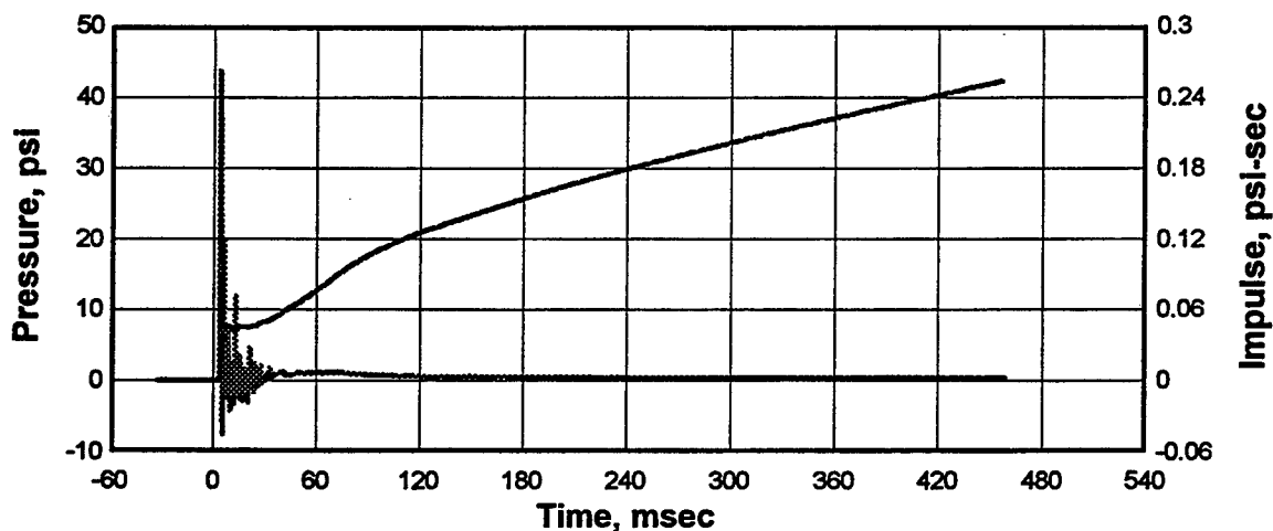
Figure E10. Pressure and impulse-time histories, free-field Gage AB-12 on the surface of the ground at a horizontal distance of 1.80m from the portal, Experiment 5.
