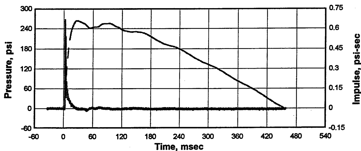
Figure C8. Total pressure and impulse-time histories, Gage AB-9 on probe mount at horizontal distance of 4.30 m from the rear wall of the detonation chamber, Experiment 3.
