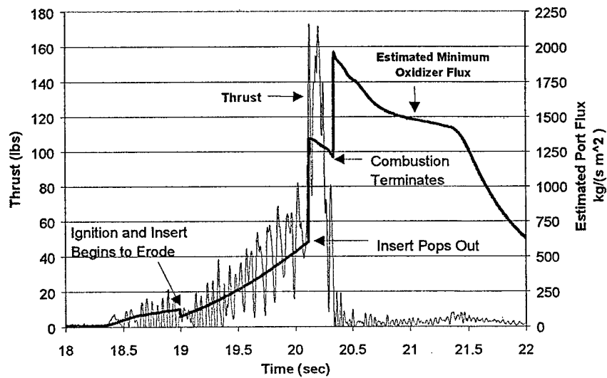
Figure 9: Combustion terminates with peroxide still flowing. Possibly caused by high oxidizer flux (greater than 700) through the port.
