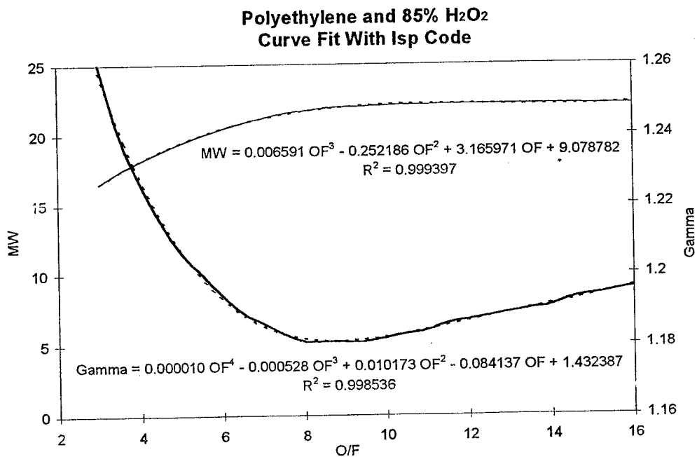
Figure 4: Chamber molecular weight (MW) and isentropic parameter (γ) as a function of peroxide to polyethylene mass ratio.
