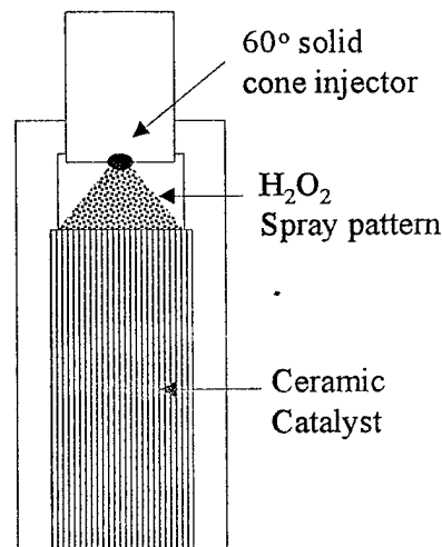
Figure 2: Axial flow catalyst design.
