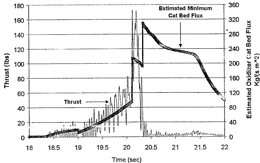
Figure 10: Visible liquid (peroxide) noticed in exhaust gases after flameout. Possibly caused by high (above 250) oxidizer flux rate through the cat bed.
