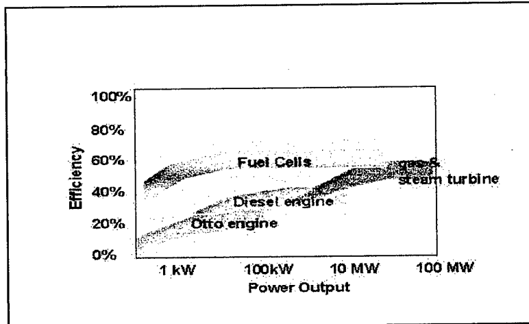
Figure 1.1 Generation Efficiencies [9]
