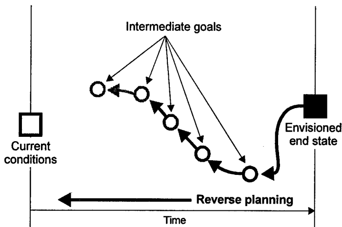
Figure 5. Reverse planning.
