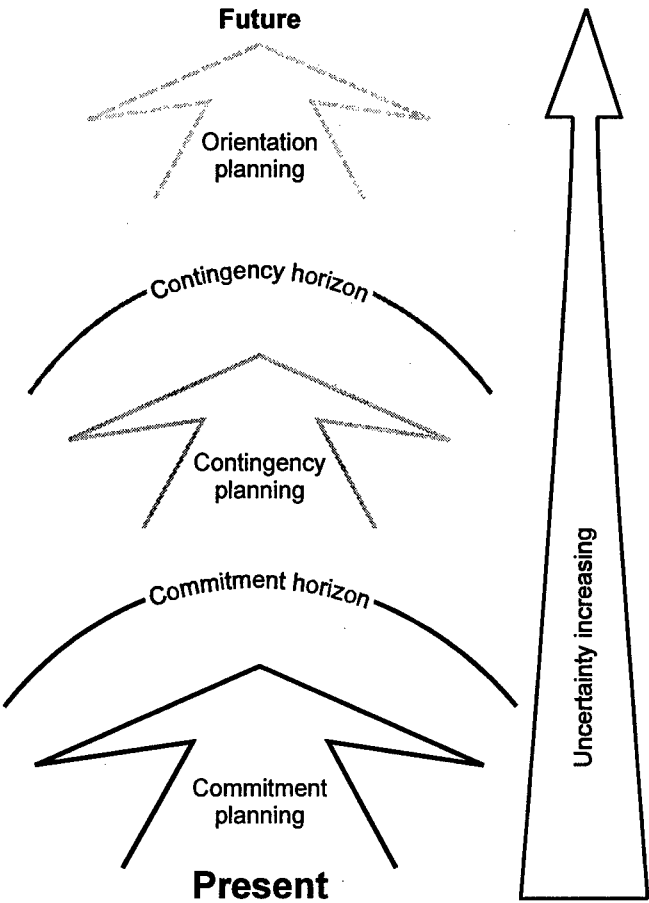
Figure 6. Planning horizons.
