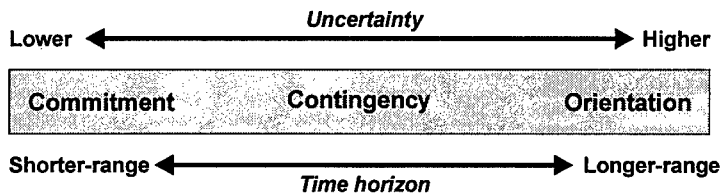
Figure 3. Planning modes.
