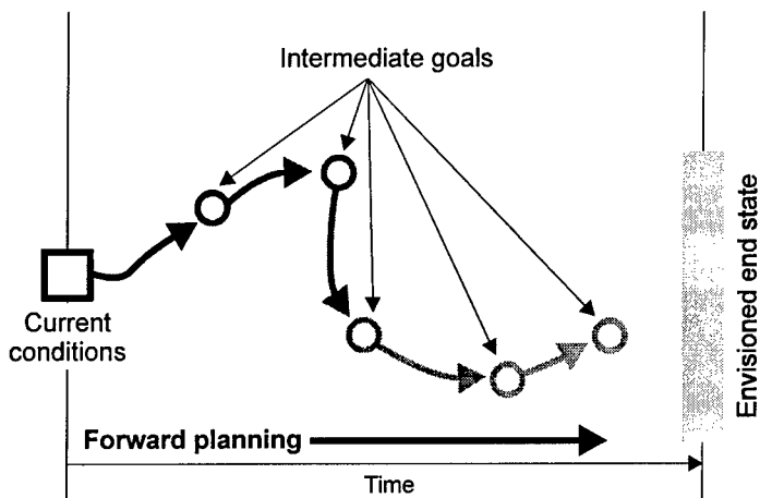
Figure 4. Forward planning.
