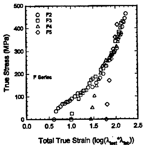
ISOTACTIC POLYPROPYLENE
