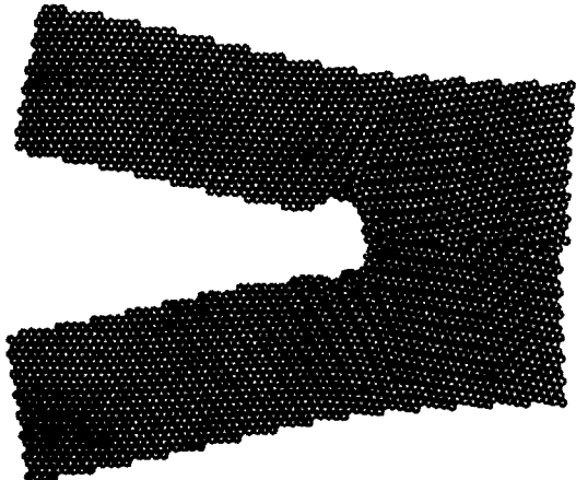
Figure 1. Crack tip configuration for a [111](123) grain boundary at a loading twice the Griffith value.
