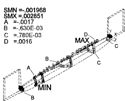
Figure 2. Distribution of mass flux divergence in an aluminum-pad-metallization (in 1/\mu\text{m}^3\text{s} ).
