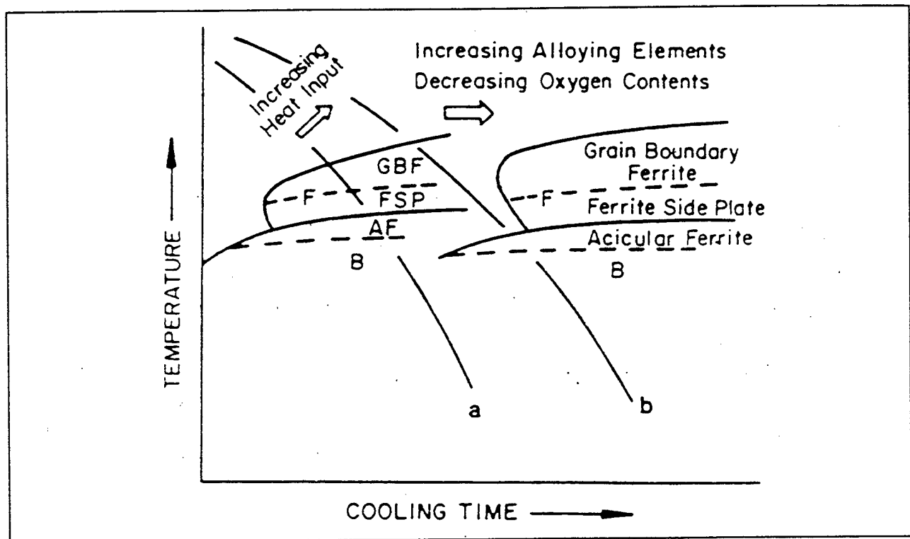
Figure 2-6. CCT diagram showing effects of increasing heat input and alloying [Ref. 1].
