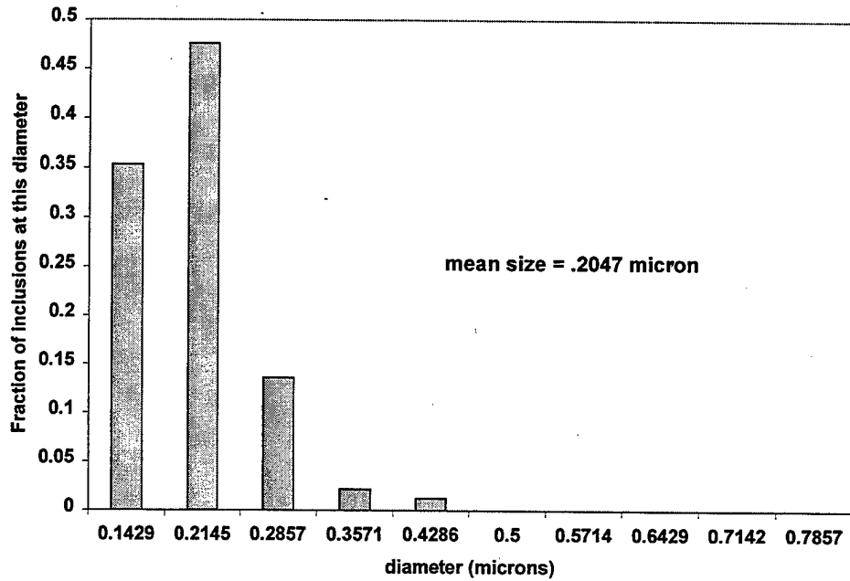
Figure 4-10. Inclusion Distribution for Sample Y and Sample Z.
