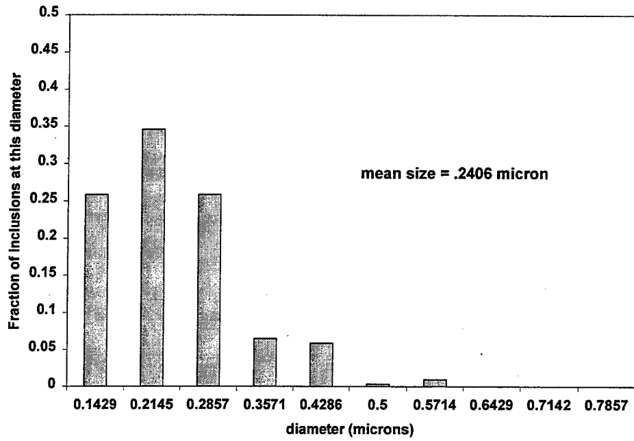
Figure 4-11. Inclusion Distribution for Sample V.
