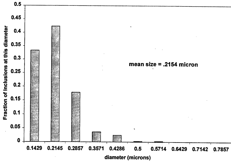
Sample Z Inclusion Distribution
