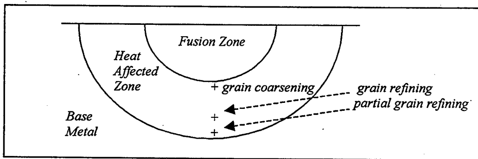
Figure 2-2. Sketch of single pass weld microstructure [Ref. 1].
