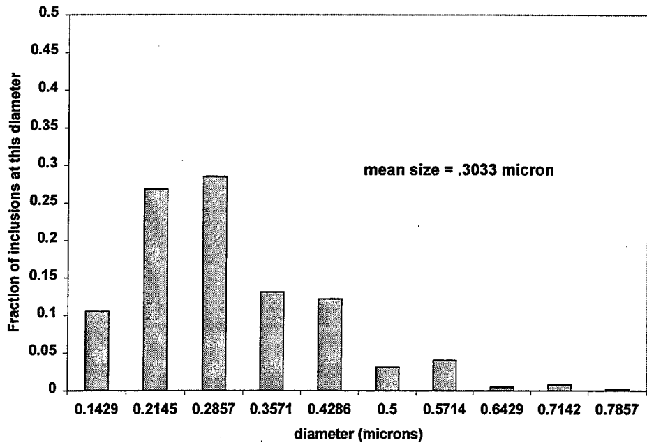
Sample O Inclusion Distribution
