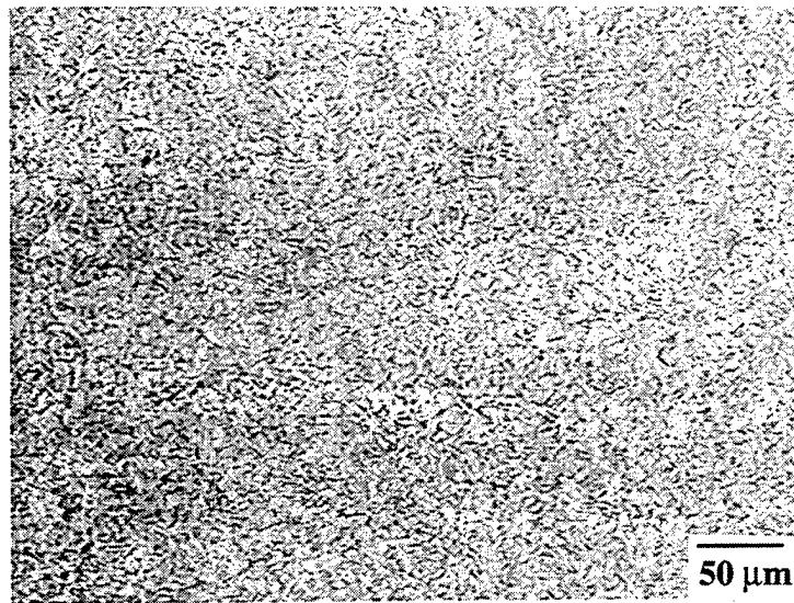
Figure 4-6. Optical micrograph of re-austenitized region for Sample W.
