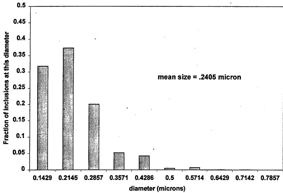
Sample W Inclusion Distribution
