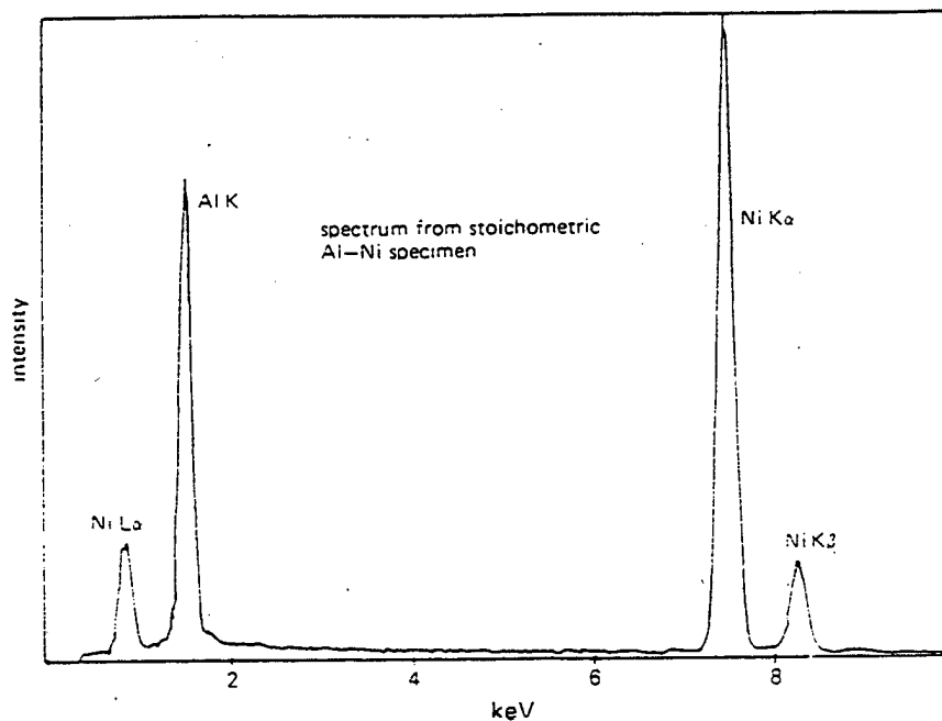
Figure 3-6. Typical EDX spectrum.
