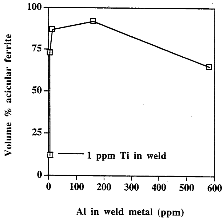
Figure 4-13. Volume percent acicular ferrite vs. weld metal aluminum. (The errors for both axes are less than the symbol size)
