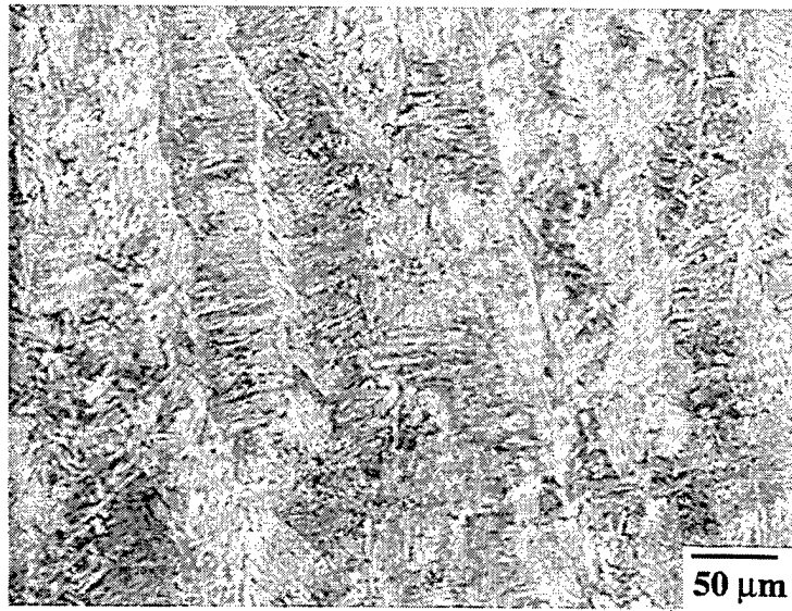
Figure 4-3. Optical micrograph of final weld pass for Sample O.
