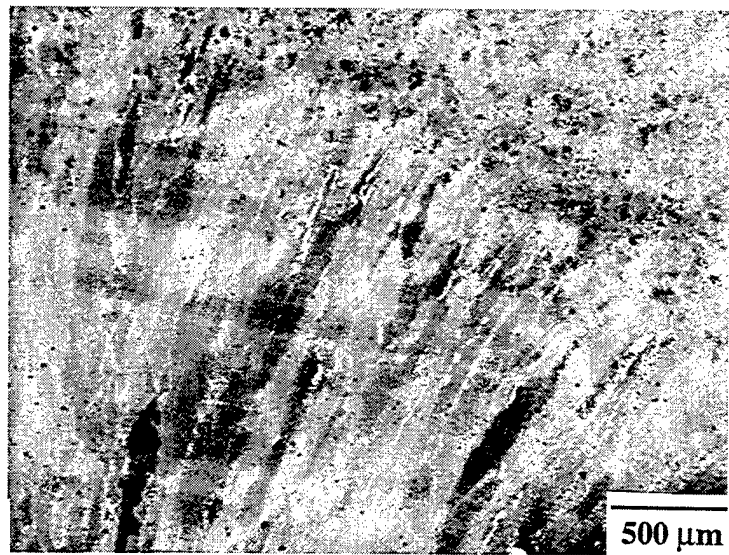
Figure 4-2. Optical micrograph of final weld pass for Sample W.
