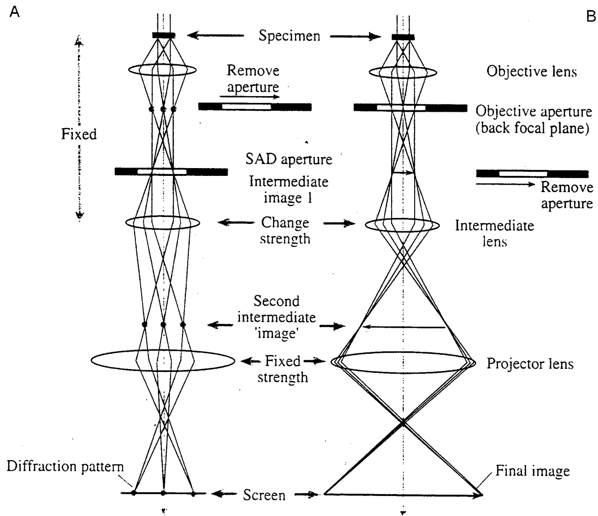
Figure 3-4. Schematic of TEM projecting (a) diffraction patterns and (b) imaging onto a fluorescent screen [From Ref. 45].
