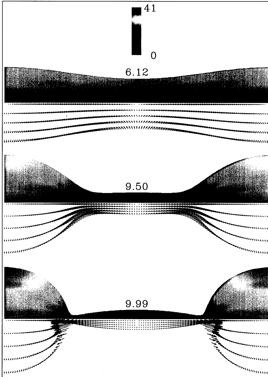
Figure 11: Pressure distribution and velocity vectors for a non-evaporating jet, Re=200 , k=0.7 , \varepsilon_0=0.05 , \beta=0 , s=10^{-3} .
