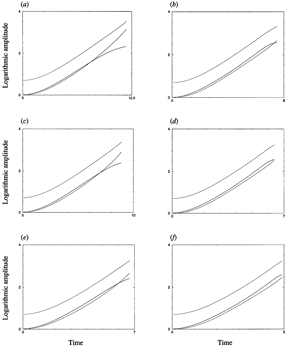
Figure 5: Variation of the amplitude of the neck (black), swell (red), and their logarithmic difference (green), Re=200 , \epsilon_o=0.5 , s=10^{-3} : (a) k=0.4 , \beta=10^{-2} ; (b) k=0.7 , \beta=10^{-2} ; (c) k=0.4 , \beta=2 \times 10^{-2} ; (d) k=0.7 , \beta=2 \times 10^{-2} ; (e) k=0.4 , \beta=3 \times 10^{-2} ; (f) k=0.7 , \beta=3 \times 10^{-2} .
