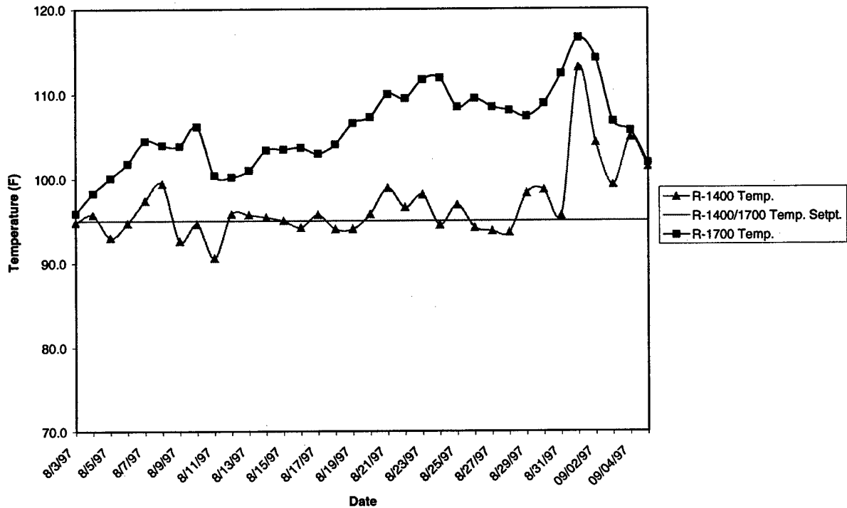
Figure 11. Reactor Temperature during Series Operation
