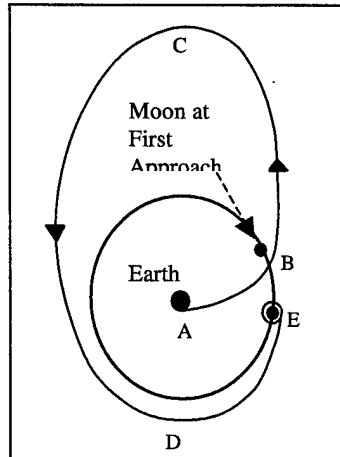
Figure 2 – Ballistic Capture Transfer
