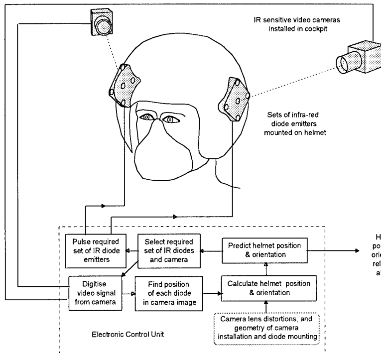
Figure 2.2-3. Schematic summarising a modern optical head tracker
