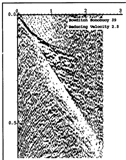
Figure 1 (above) A poor sonobuoy record. Good enough to obtain a velocity function, but exhibiting a weak signal and the “AGC” effect described below.
