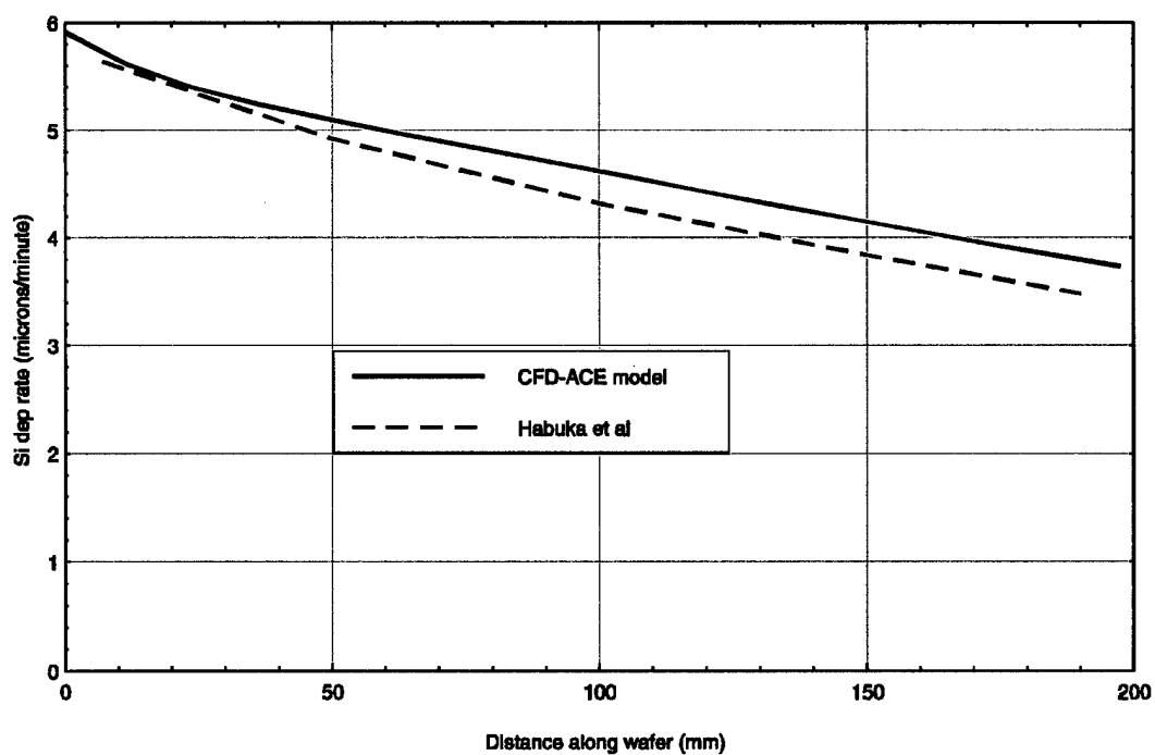
Figure 15. Deposition profile along flow direction. Comparison with Habuka, et al [52].
