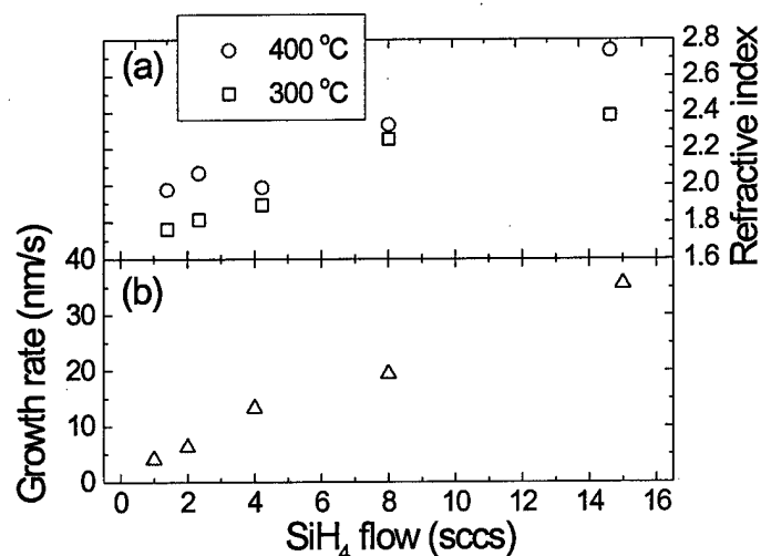
Figure 6: Refractive index (a) and growth rate (b) as a function of SiH 4 flow for films deposited at substrate temperatures of 300 and 400 °C and with a H 2 flow of 5 sccs.
