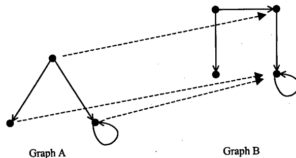
Figure A-2. Graphical depiction of two graphs and a graph morphism between them
