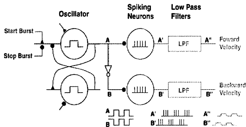
Figure 1 On chip functions of the CPG chip.
