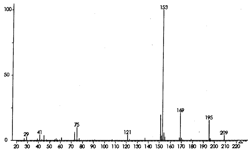
Figure A.3: Sec-butyl trimethylsilyl methylphosphonate (MW 224).
