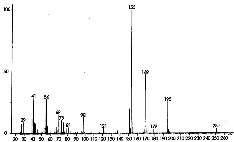
Figure A.11: 1-Methylhexyl trimethylsilyl methylphosphonate (MW 266).
