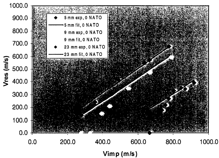
Figure C.2: Results of 5.3 g. FSPs on the E-glass fibre & vinyl ester plates.
