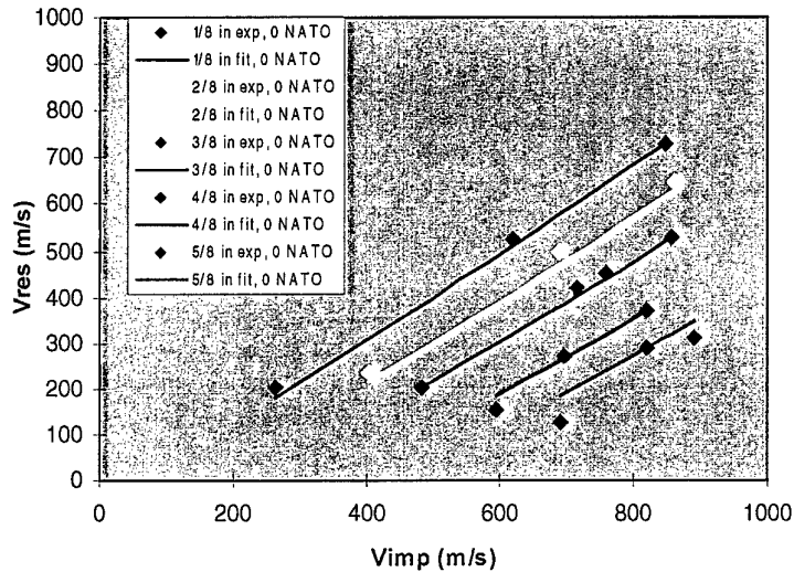
Figure B.1: Results of 1.1 g. FSPs for the Hercules AS4/3501 plates.
