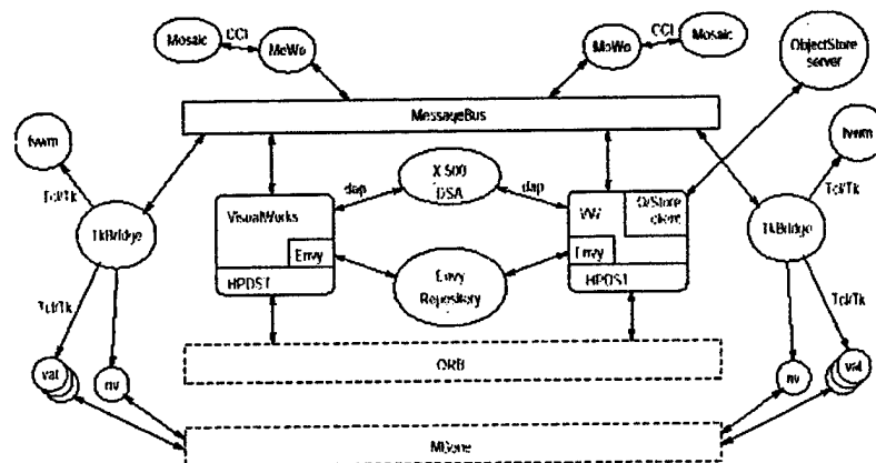
Figure 1 wOrlds Architecture
