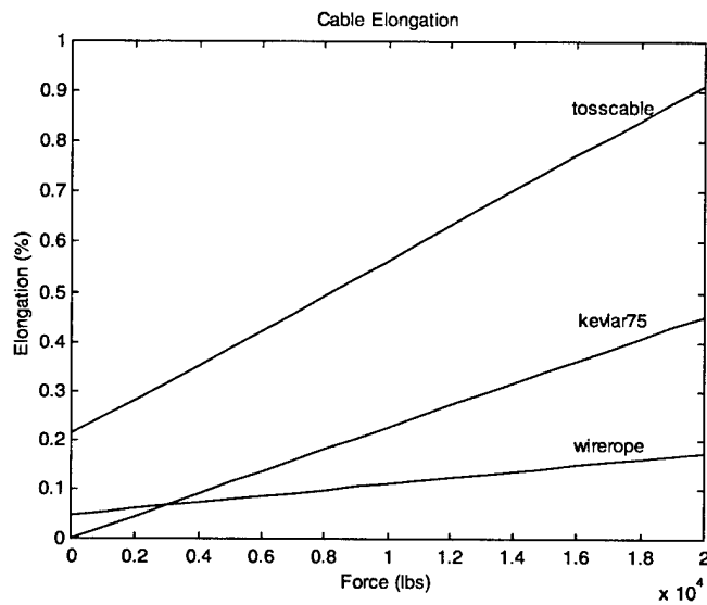
Figure 4. Elongation of cable under load.
