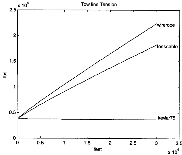
Figure 16. Towline tension at 2 knots.
