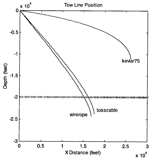
Figure 13. Towline position at 2 knots. Note that the neutral kevlar cable does not reach the desired 20,00-foot depth.
