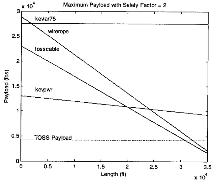
Figure 3. Payload capacity as a function of length.
