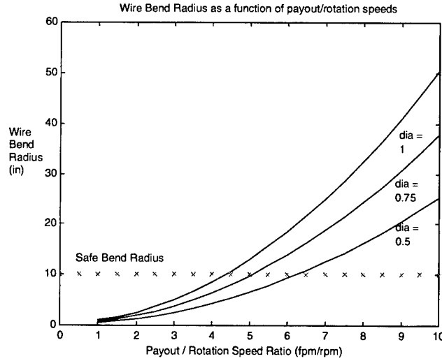
Figure 10. Detailed effective wrapped cable bend radius.
