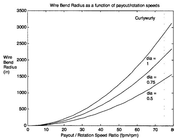
Figure 9. Effective bend radius of wrapped cable.
