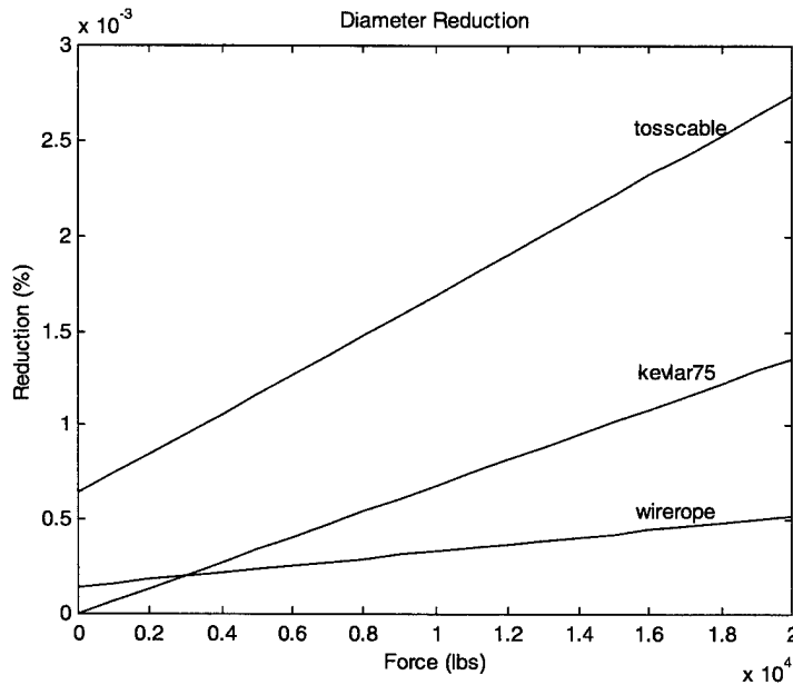
Figure 5. Diameter reduction under load.
