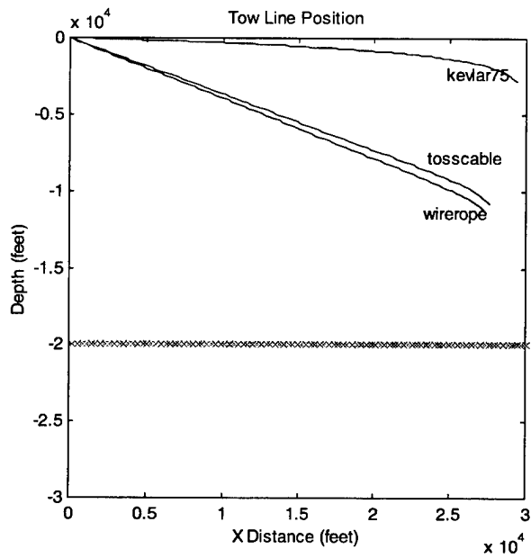
Figure 14. Towline position at 5 knots. Note that no payloads reach the "desired" 20,000-foot depth.
