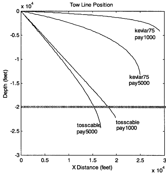
Figure 15. Towline position at 2 knots as a function of payload weight.
