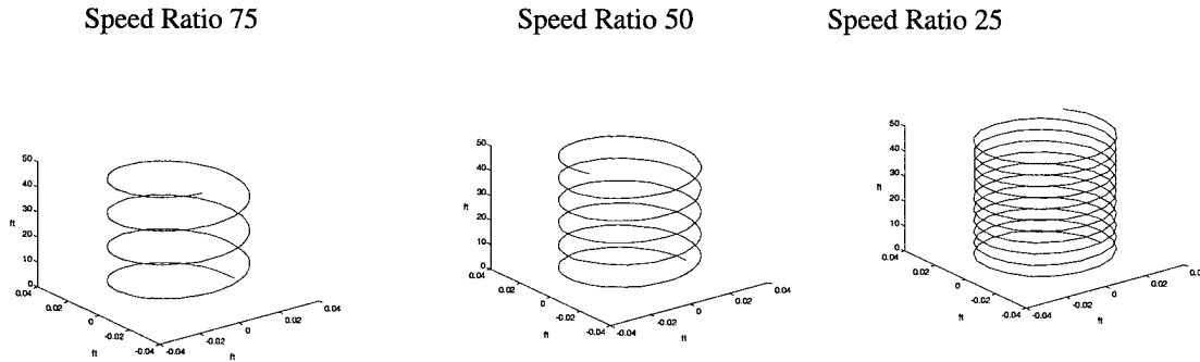
Figure 8. Relative wrapping densities as a function of speed ratios of 75, 50, and 25. Note that the speed ratio is proportional to the actual pitch length.
