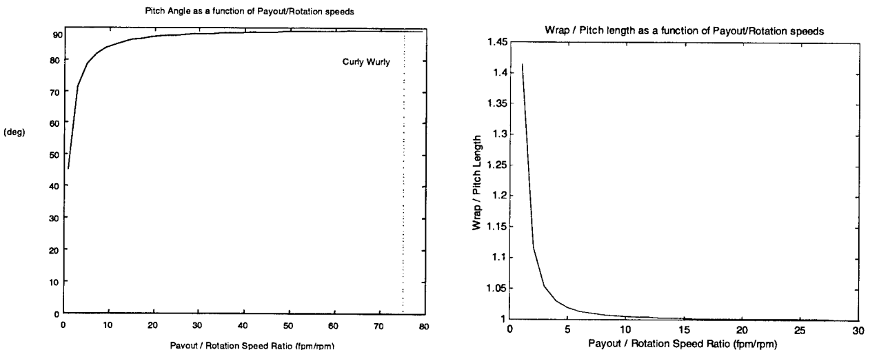
Figure 7. Pitch angle and pitch length as a function of payout versus wrapping speeds.
