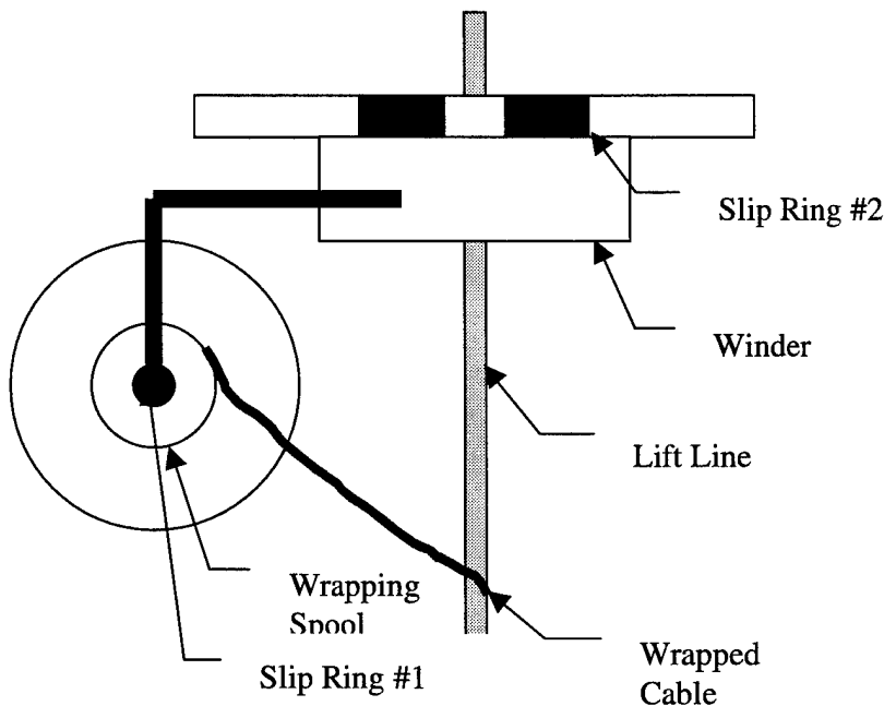
Figure 18. Curly Wurly configuration (front view).
