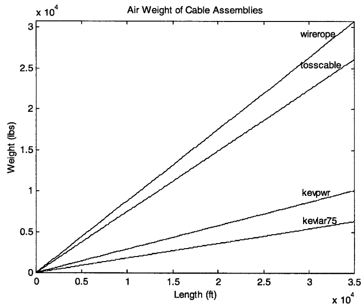
Figure 2. Cable assembly weight as a function of length.
