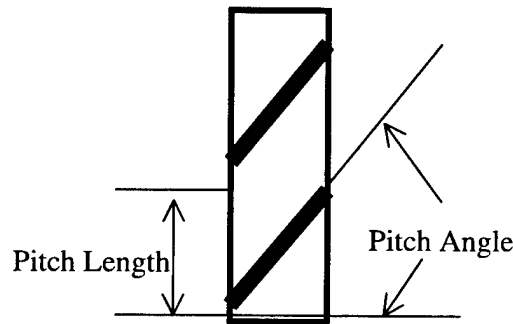
Figure 6. Pitch length and angle of wrapped cable.
