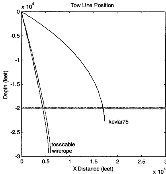
Figure 12. Towline position at 1 knot.
