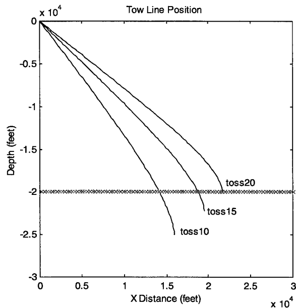
Figure 17. Effect of increasing cable drag coefficients on tow body position. Toss10 has a Cd of 1.0, toss15 has a Cd of 1.5, and toss20 has a Cd of 2.0.
