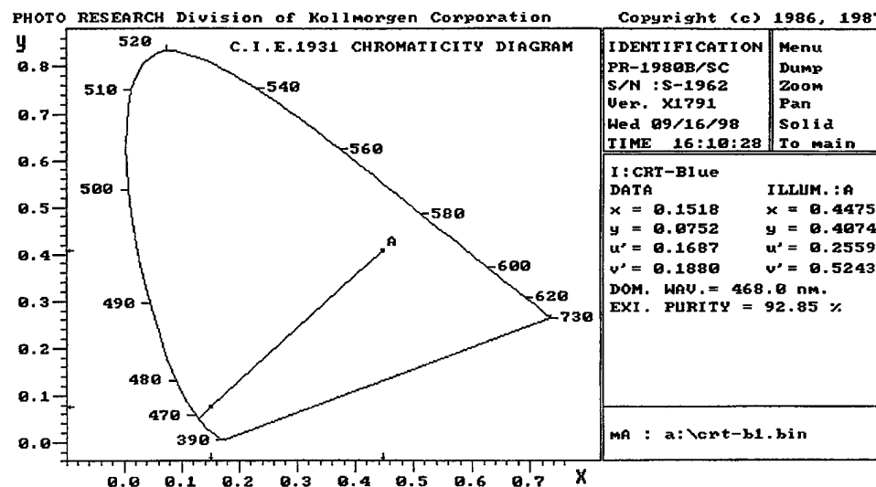
Figure 23. CIE 1931 chromaticity diagram for CRT—blue.
