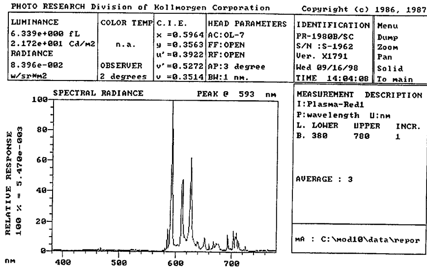
Figure 6. Plasma spectral scan—red.
