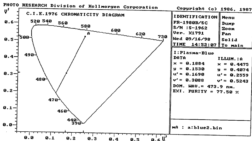
Figure 14. CIE 1976 chromaticity diagram for plasma display—blue.
