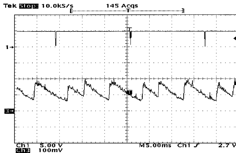
Figure 4. Luminance response of plasma display with acquisition mode at average 15.
