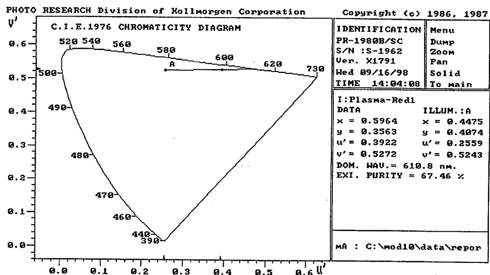
Figure 12. CIE 1976 chromaticity diagram for plasma display—red.
