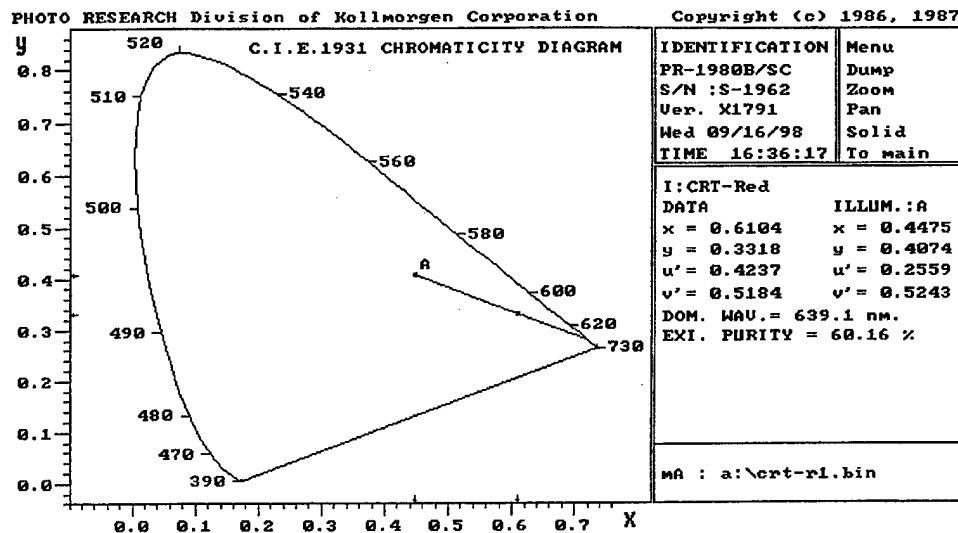
Figure 21. CIE 1931 chromaticity diagram for CRT—red.
