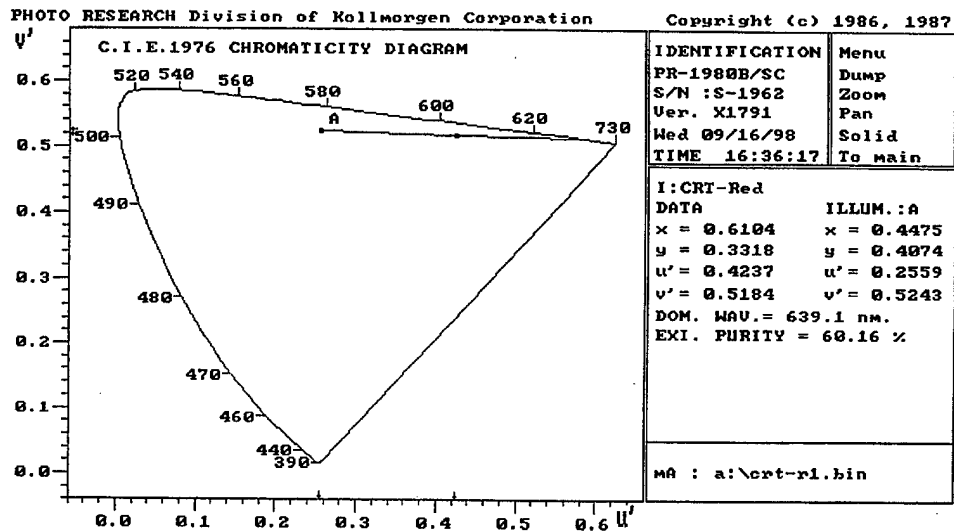
Figure 18. CIE 1976 chromaticity diagram for CRT—red.
