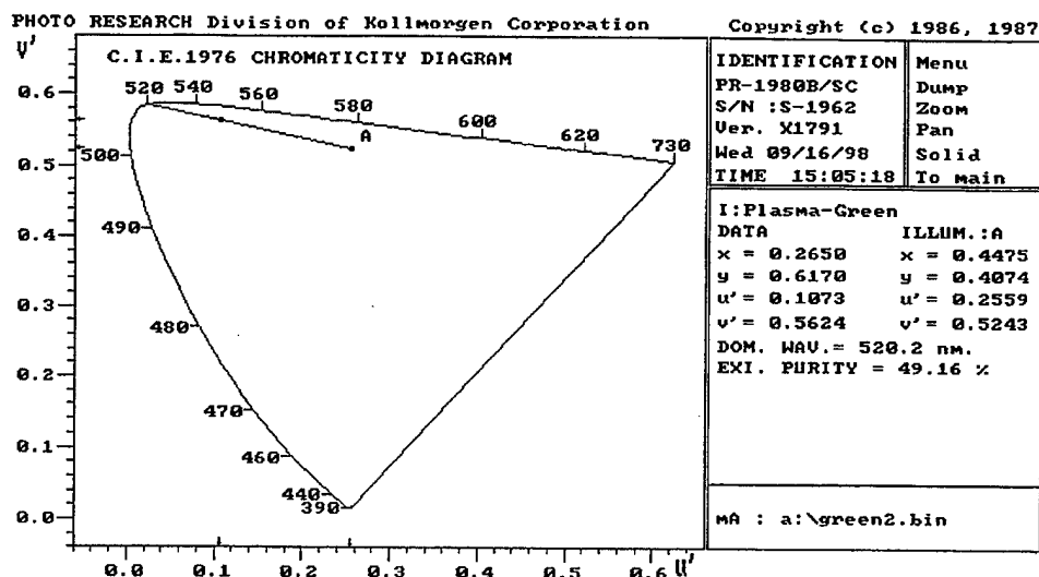
Figure 13. CIE 1976 chromaticity diagram for plasma display—green.
