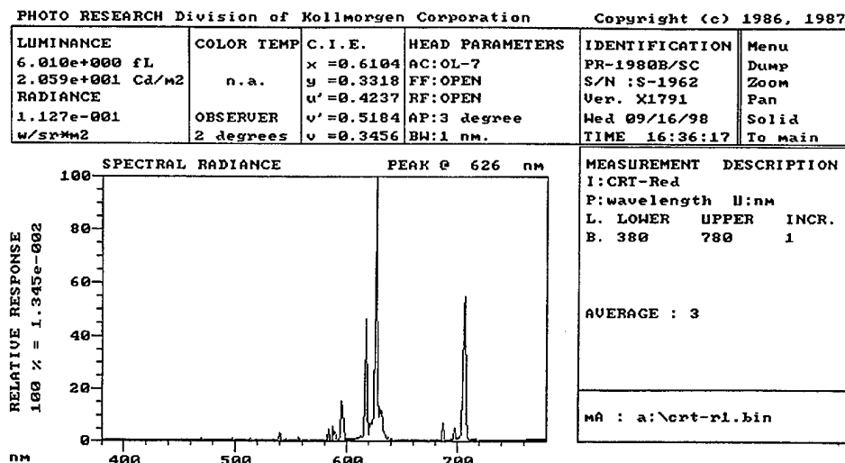
Figure 9. CRT spectral scan—red.
