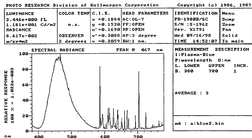
Figure 8. Plasma spectral scan—blue.
