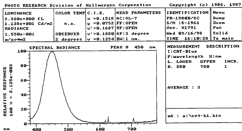
Figure 11. CRT spectral scan—blue.
