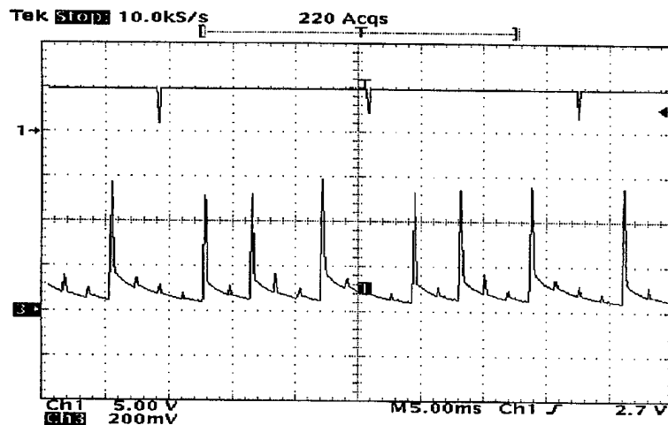
Figure 5. Luminance response of plasma display with acquisition mode at high resolution.
