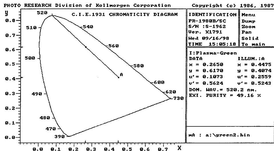
Figure 16. CIE 1931 chromaticity diagram for plasma display—green.
