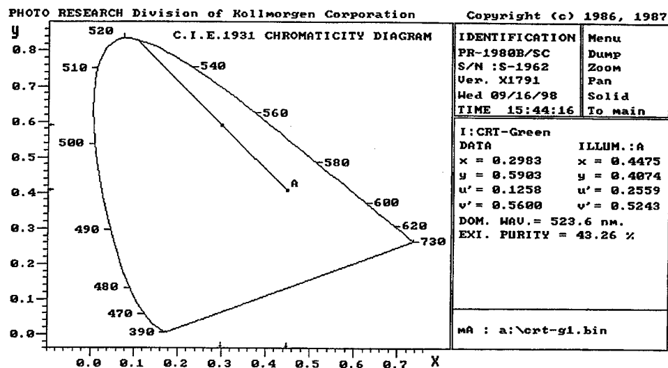
Figure 22. CIE 1931 chromaticity diagram for CRT—green.
