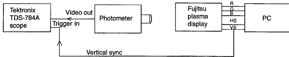
Figure 2. Measurement setup for luminance response characteristic.
