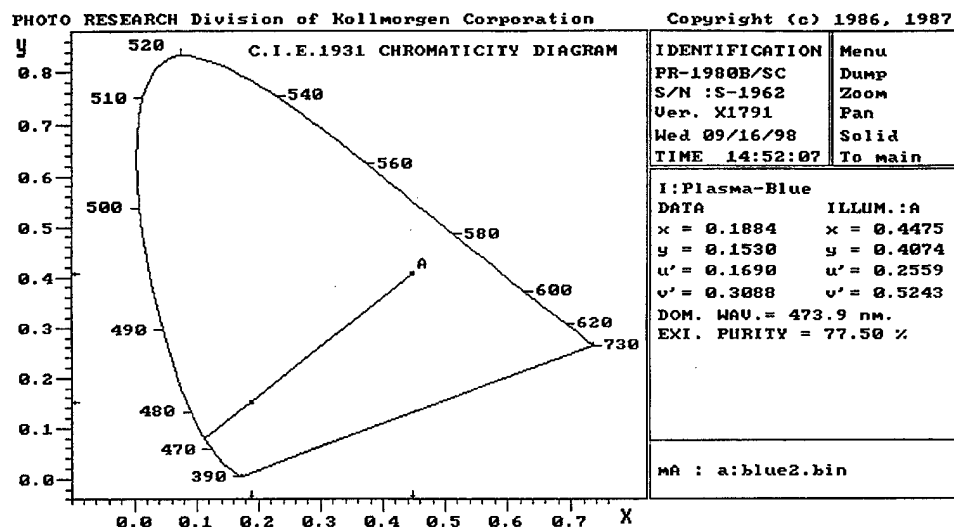
Figure 17. CIE 1931 chromaticity diagram for plasma display—blue.
