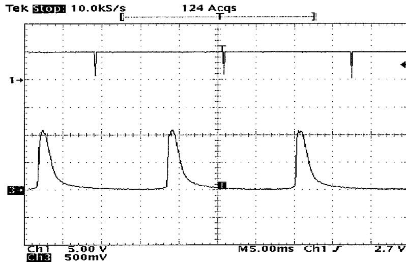
Figure 3. Luminance response of typical CRT display with acquisition mode at average 15.
