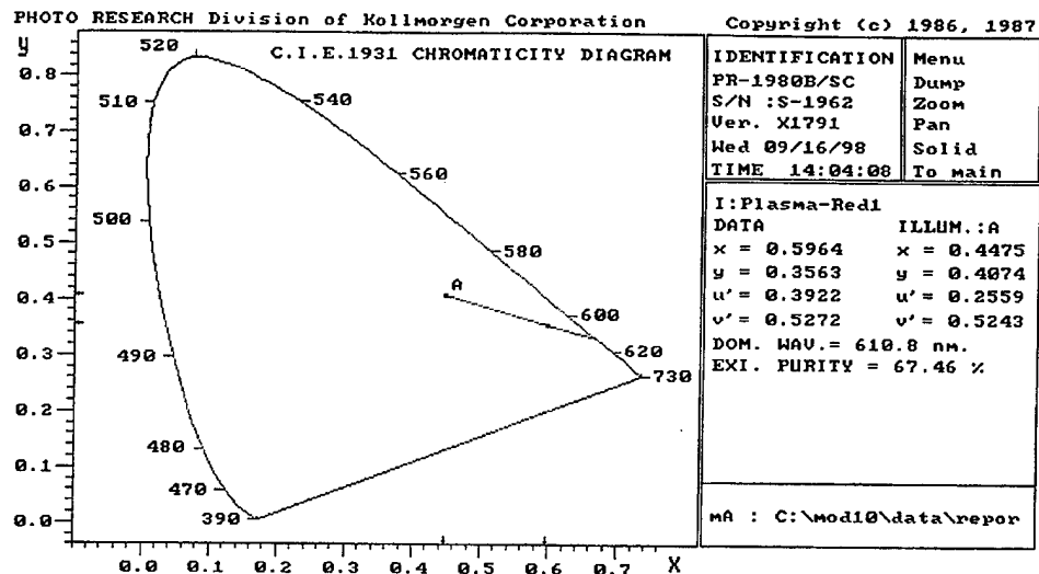
Figure 15. CIE 1931 chromaticity diagram for plasma display—red.
