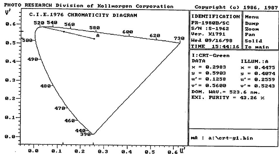
Figure 19. CIE 1976 chromaticity diagram for CRT—green.
