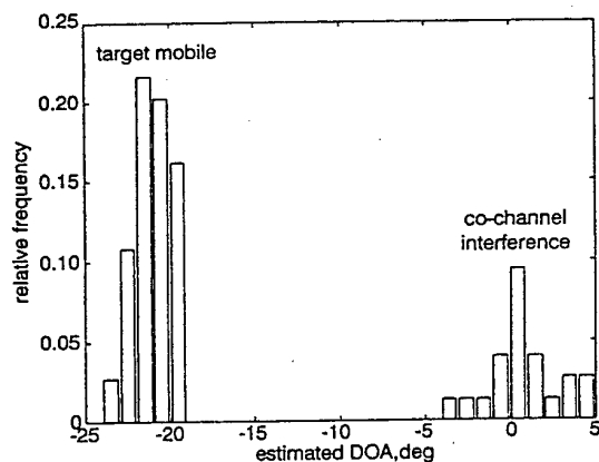
Fig. 1 Histogram of DOA estimates over 2s period
