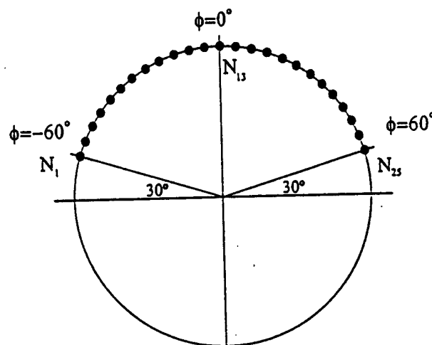
Figure 2 Geometry of the circular arc array
