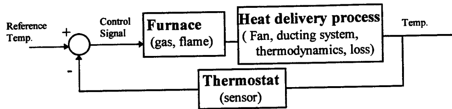
Figure 1.1 - Typical Control System for Space Heating
