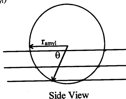
Figure 3.24 - Actin Grid Forces
