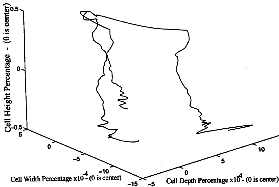
Figure 3.26 - Finite-element Model of Falling Amyloplasts
