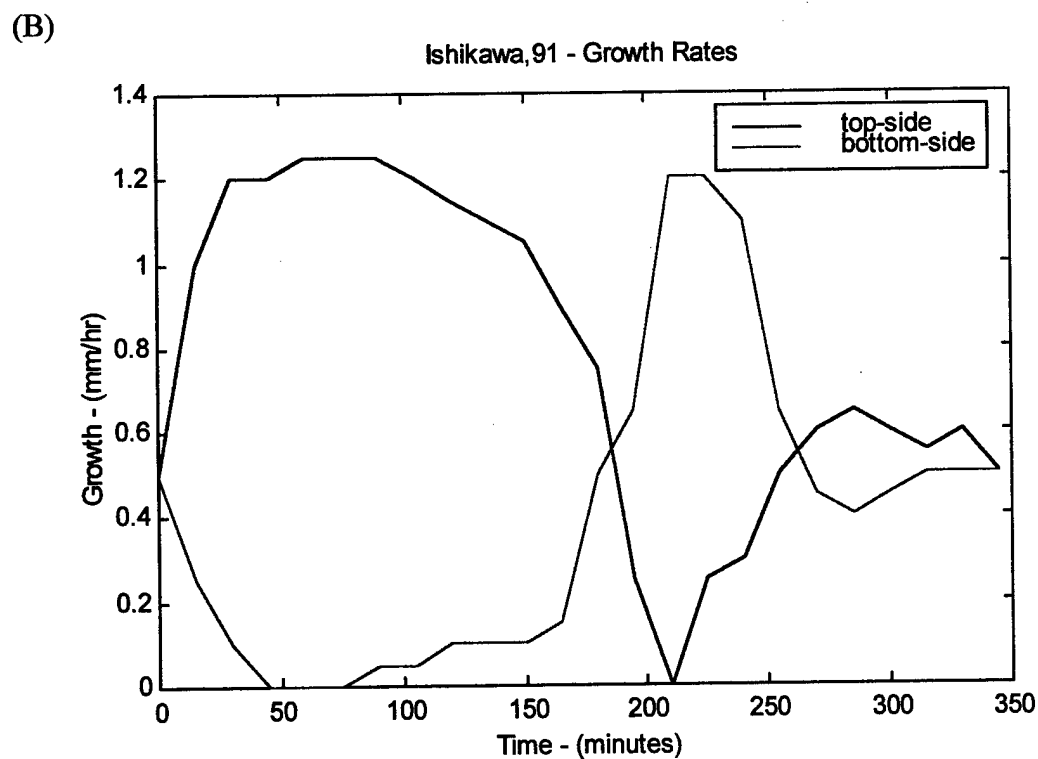
Figure 4.4 - Overall Elongation Rates on the Top and Bottom of the Maize Root Linear interpolation between actual data points every 30 minutes for (A)(Pilet, 1989) and every 15 minutes for (B)(Ishikawa et al. , 1991).
