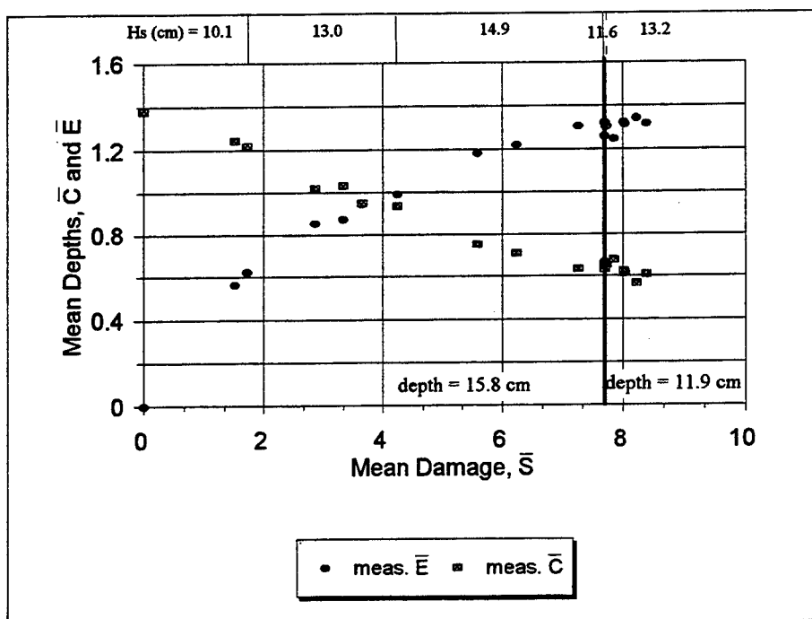
Figure 5.25. Mean damage versus mean maximum eroded depth and mean minimum cover depth for Series C'
