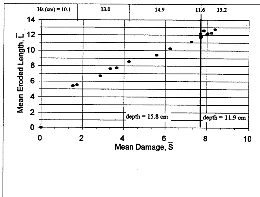
Figure 5.27. Mean damage versus mean maximum eroded length for Series C'
