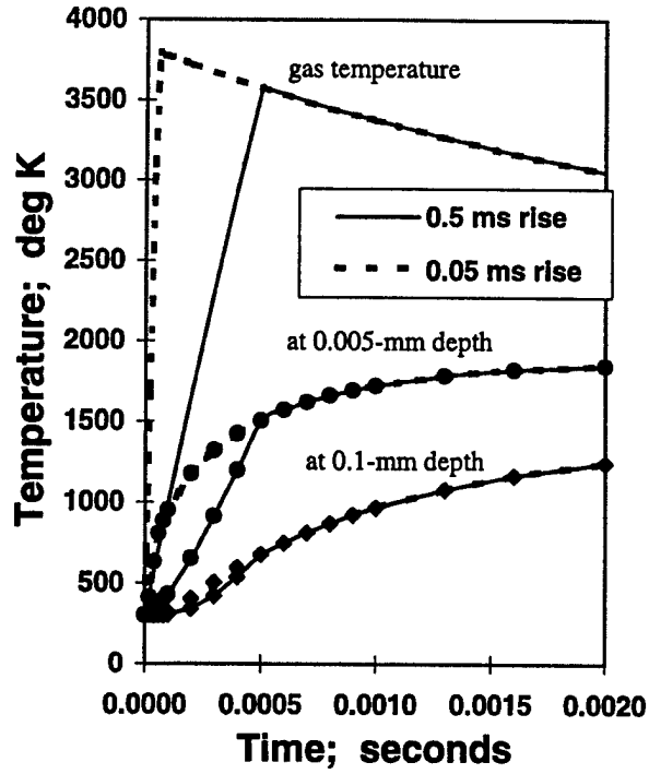
Figure 9. Effect of temperature rise time due to round passage on chromium temperature at various times and depths for cannon A.
