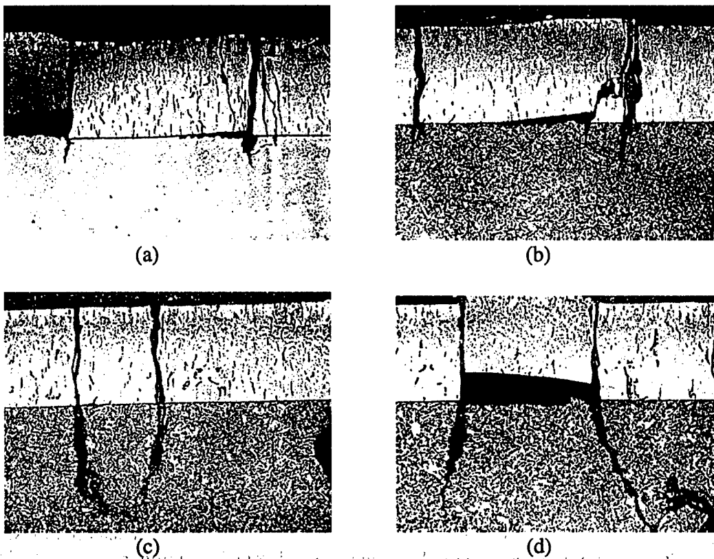
Figure 2. Polished and etched section from near-bore region of cannon B (130X). Figures 2(a) and (b) are longitudinal orientation at 1.5-m forward of breech end of tube. Figures 2(c) and (d) are transverse orientation at 0.7-m forward of breech end of tube.
