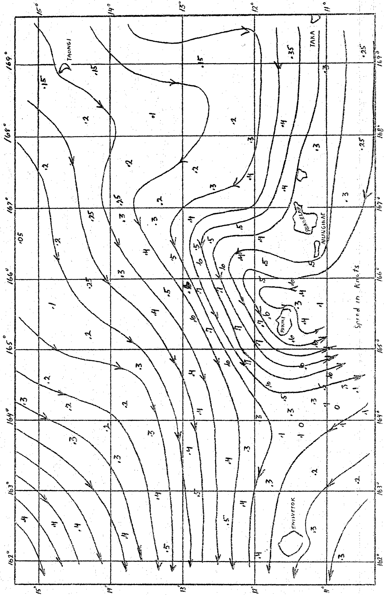
DIRECTION AND SPEED OF CURRENTS AT 75 METERS DEPTH
