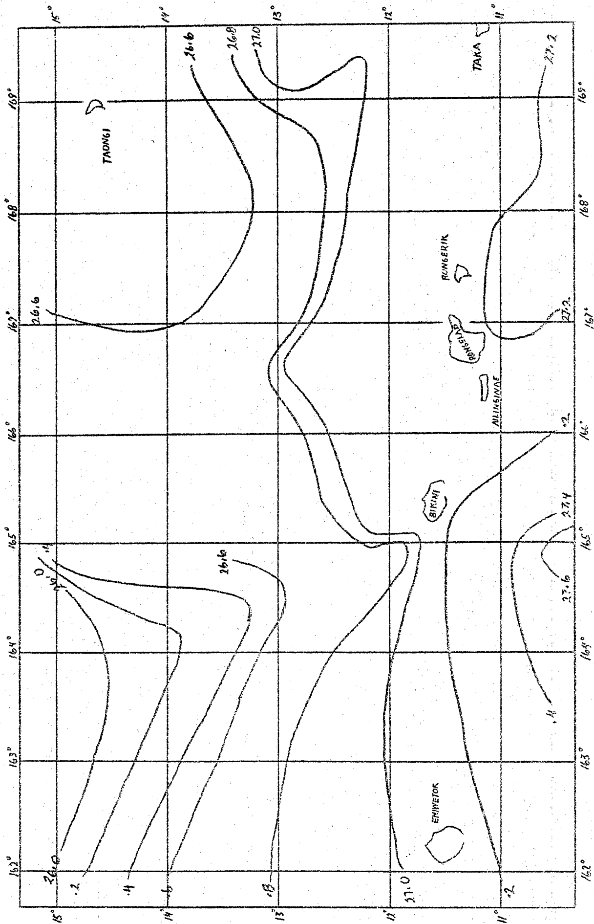
SURFACE TEMPERATURE (C)
