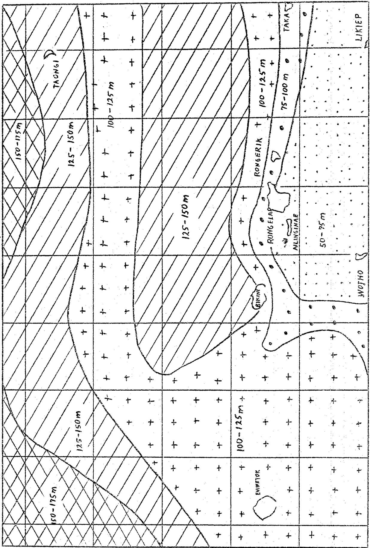
DEPTH OF MOST STABLE 25 METER LAYER
