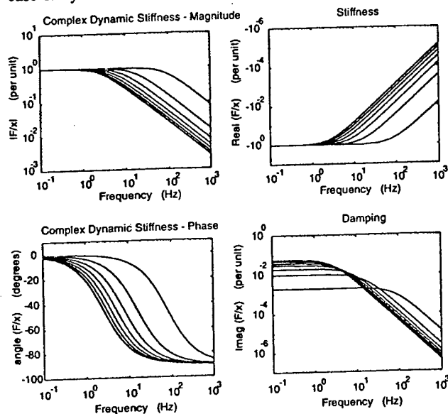
Fig. 12 Radial force frequency response to eccentricity variations.
