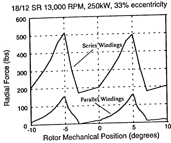
Fig. 11 Dynamic radial force comparison for voltage and current source excitation.
