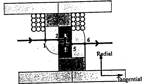
Fig. 4 Application of the Maxwell Stress Tensor in the calculation of radial and tangential forces.
