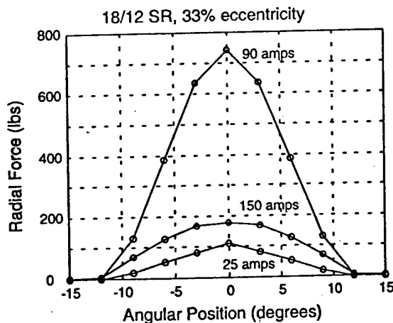
Fig. 7 Radial force—vs—pole position, 18/12 SRM, 33% gap offset in rotor position, FEA results.
