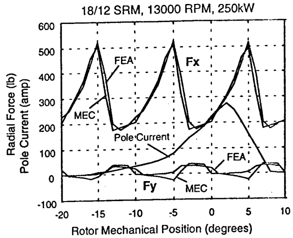
Fig. 10 Radial force with dynamic current source excitation, 18/12 SR machine with 33% gap offset.
