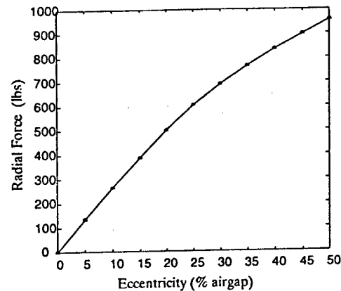
Fig. 8 Radial force—vs—eccentricity, 18/12 SRM, 90 amps and 100% alignment.
