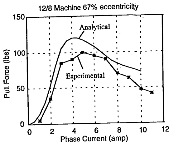
Fig. 14 Predicted and measured radial force -vs- current for a 12/8 SR test machine.
