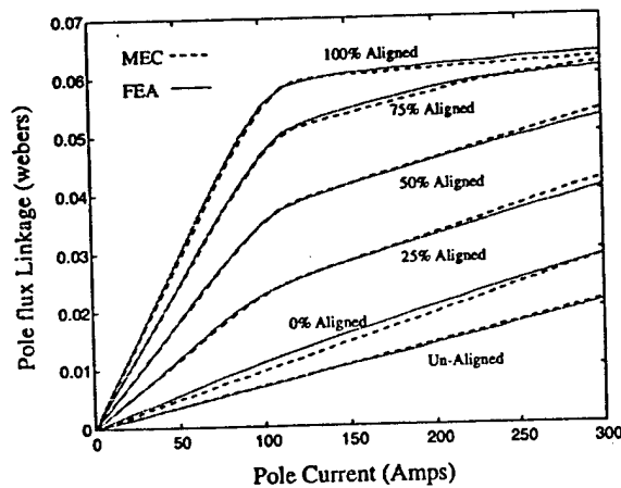
Fig. 3 Flux Linkage Characteristics, 18/12 SRM - Comparison of MEC & FEA
