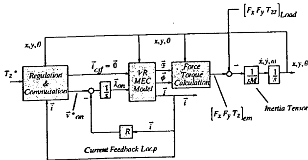
Fig. 9 Dynamic simulation model of the SR system.
