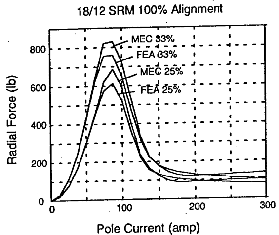
Fig. 5 Radial force -vs- pole current, 18/12 SRM, 25% & 33% gap offset in rotor position.
