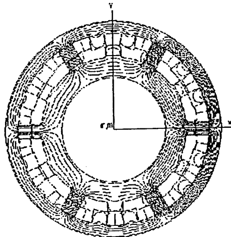
Fig. 2 FEA Flux plot for an 18/12 SRM with a 33% gap rotor offset position.
