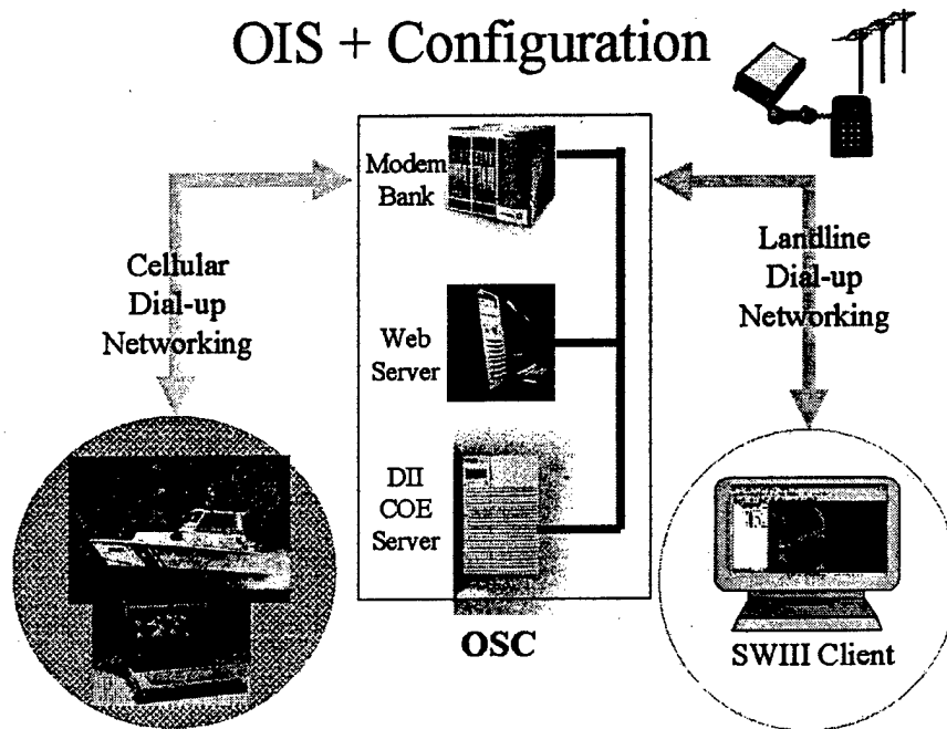
Figure 20: OIS+ Conceptual Configuration
