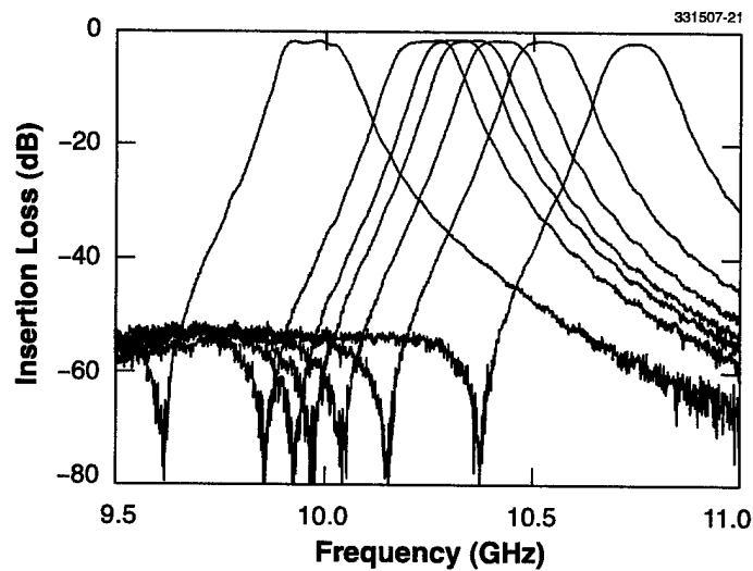
Figure 6-2. Insertion loss vs frequency for the filter of Figure 6-1, for several values of applied magnetic field from zero to approximately 300 G. The materials are niobium superconductor on G1210.
