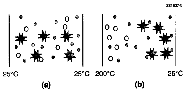
Figure 3-5. (a) Gaseous constituents are uniformly mixed at constant temperature. (b) Thermal gradient causes constituents to separate. Solid circles represent the carrier gas, air or nitrogen; open circles represent a constituent of lower molecular weight; and stars represent a constituent of higher molecular weight.
