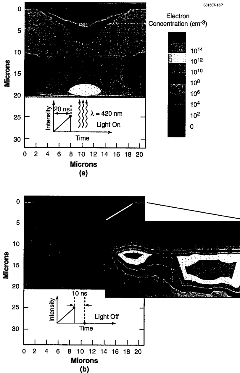
Figure 5-1. Summary of the transient analysis methodology. Electron concentration contours are plotted during a (a) light-on, (b) light-off sequence, and total collected charge is monitored as a function of time. Collection electrodes located on the front side surface are 10\ \mu\text{m} in width separated by a distance d\ (\mu\text{m}) . The inset shows that all of the charge is eventually collected in the well.
