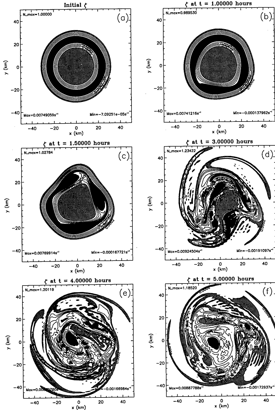
Figure 4.12: SS model vorticity evolution for the ring experiment from t = 0 to 5 h. In each panel, a 100 \text{ km} \times 100 \text{ km} subset of the entire domain is plotted. The lowest contour level is 2.0 \times 10^{-4} \text{ s}^{-1} with the remaining contour levels beginning at 1.0 \times 10^{-3} \text{ s}^{-1} in increments of 1.0 \times 10^{-3} \text{ s}^{-1} . Grey indicates 2.0 \times 10^{-4} \text{ s}^{-1} \leq \zeta \leq 1.0 \times 10^{-3} \text{ s}^{-1} , and black indicates \zeta \geq 6.0 \times 10^{-3} \text{ s}^{-1} .
