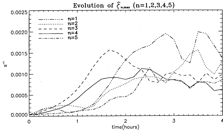
Figure 4.9: Evolution of the maximum of the eigenfunction \hat{\zeta}_{n,\max} for wavenumbers 1 through 5 from t = 0 to t = 4 h.
