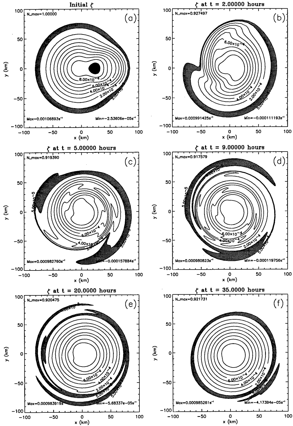
Figure 3.10: Wave-mean flow evolution of the perturbed monopole as simulated in the SS model. In each panel, a 200 \text{ km} \times 200 \text{ km} subset of the entire domain is plotted. The lowest contour level is 5.0 \times 10^{-5} \text{ s}^{-1} with the remaining contour levels beginning at 1.0 \times 10^{-4} \text{ s}^{-1} in increments of 1.0 \times 10^{-4} \text{ s}^{-1} . Grey indicates 5.0 \times 10^{-5} \text{ s}^{-1} \leq \zeta \leq 1.0 \times 10^{-4} \text{ s}^{-1} , and black indicates \zeta \geq 10.0 \times 10^{-4} \text{ s}^{-1} .
