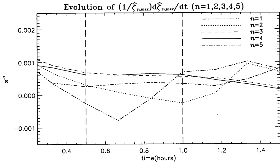
Figure 4.10: Evolution of the growth rates (1/\hat{\zeta}_{n,\max})d\hat{\zeta}_{n,\max}/dt for wavenumbers 1 through 5 from t = 0.25 to t = 1.5 h.
