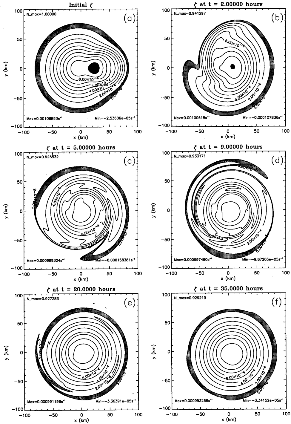
Figure 3.9: Linear evolution of the perturbed monopole as simulated in the SS model. In each panel, a 200 \text{ km} \times 200 \text{ km} subset of the entire domain is plotted. The lowest contour level is 5.0 \times 10^{-5} \text{ s}^{-1} with the remaining contour levels beginning at 1.0 \times 10^{-4} \text{ s}^{-1} in increments of 1.0 \times 10^{-4} \text{ s}^{-1} . Grey indicates 5.0 \times 10^{-5} \text{ s}^{-1} \leq \zeta \leq 1.0 \times 10^{-4} \text{ s}^{-1} , and black indicates \zeta \geq 10.0 \times 10^{-4} \text{ s}^{-1} .
