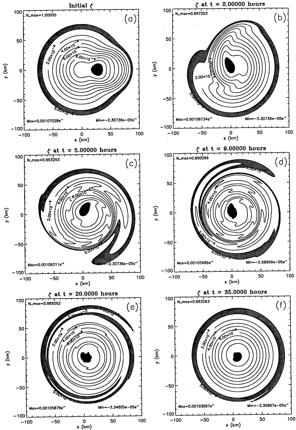
Figure 3.4: FD model vorticity evolution for the perturbed monopole experiment. In each panel, a 200 km \times 200 km subset of the entire domain is plotted. The lowest contour level is 5.0 \times 10^{-5} \text{ s}^{-1} with the remaining contour levels beginning at 1.0 \times 10^{-4} \text{ s}^{-1} in increments of 1.0 \times 10^{-4} \text{ s}^{-1} . Grey indicates 5.0 \times 10^{-5} \text{ s}^{-1} \leq \zeta \leq 1.0 \times 10^{-4} \text{ s}^{-1} , and black indicates \zeta \geq 10.0 \times 10^{-4} \text{ s}^{-1} .
