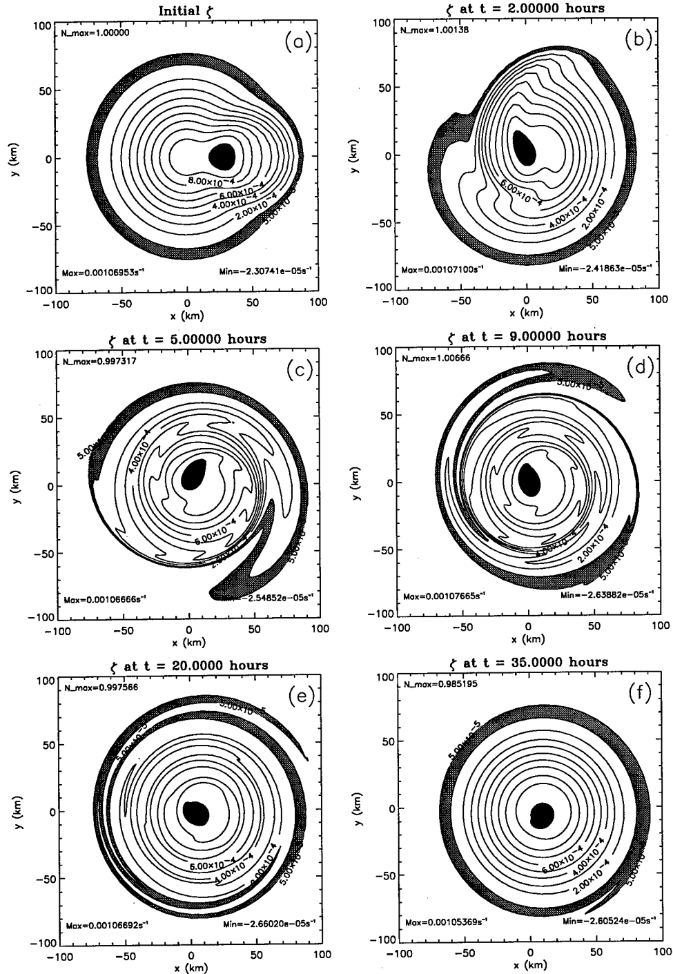
Figure 3.6: SS model vorticity evolution for the perturbed monopole experiment. In each panel, a 200 km \times 200 km subset of the entire domain is plotted. The lowest contour level is 5.0 \times 10^{-5} \text{ s}^{-1} with the remaining contour levels beginning at 1.0 \times 10^{-4} \text{ s}^{-1} in increments of 1.0 \times 10^{-4} \text{ s}^{-1} . Grey indicates 5.0 \times 10^{-5} \text{ s}^{-1} \leq \zeta \leq 1.0 \times 10^{-4} \text{ s}^{-1} , and black indicates \zeta \geq 10.0 \times 10^{-4} \text{ s}^{-1} .
