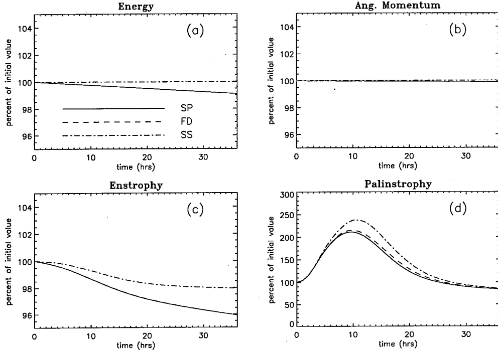
Figure 3.7: Time evolution of integrated (a) total energy ( E = \iint \frac{1}{2} \nabla \psi \cdot \nabla \psi dA ), (b) angular momentum ( AM = \iint r^2 \zeta dA ), (c) enstrophy ( V = \iint \frac{1}{2} \zeta^2 dA ), and (d) palinstrophy ( P = \iint \frac{1}{2} \nabla \zeta \cdot \nabla \zeta dA ) over the course of the run for the SP model (solid), FD model (dashed), and SS model (dash-dot). Values are normalized based on the initial value. Note the scale changes from (c) to (d). In (a), (b), and (c) the FD curve is not visible because it is covered by the SP curve.
