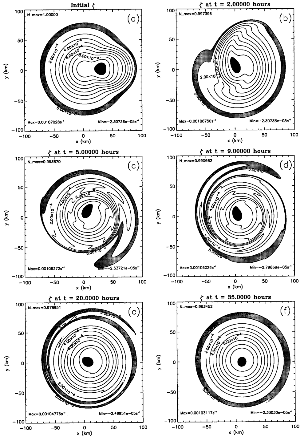
Figure 3.5: SP model vorticity evolution for the perturbed monopole experiment. In each panel, a 200 km \times 200 km subset of the entire domain is plotted. The lowest contour level is 5.0 \times 10^{-5} s^{-1} with the remaining contour levels beginning at 1.0 \times 10^{-4} s^{-1} in increments of 1.0 \times 10^{-4} s^{-1} . Grey indicates 5.0 \times 10^{-5} s^{-1} \leq \zeta \leq 1.0 \times 10^{-4} s^{-1} , and black indicates \zeta \geq 10.0 \times 10^{-4} s^{-1} .
