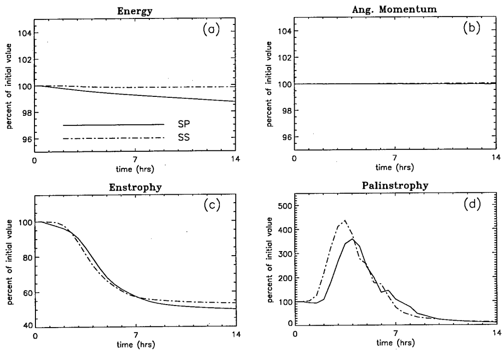
Figure 4.15: Time evolution of integrated (a) total energy ( E = \iint \frac{1}{2} \nabla \psi \cdot \nabla \psi dA ), (b) angular momentum ( AM = \iint r^2 \zeta dA ), (c) enstrophy ( V = \iint \frac{1}{2} \zeta^2 dA ), and (d) palinstrophy ( P = \iint \frac{1}{2} \nabla \zeta \cdot \nabla \zeta dA ) over the course of the run for the SP model (solid) and the SS model (dash-dot). Values are normalized based on the initial value. Note the scale changes from (b) to (c) and (c) to (d).
