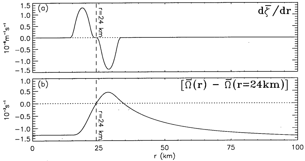
Figure 4.4: Plots of (a) gradient of storm vorticity ( d\bar{\zeta}/dr ) and (b) \bar{\Omega}(r) - \bar{\Omega}(r = 24 \text{ km}) for the modified profile. The dashed vertical line show the location where r=24 \text{ km} .
