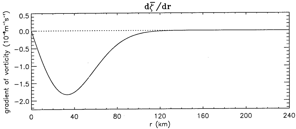
Figure 3.2: Gradient of vorticity for the monopole experiments.
