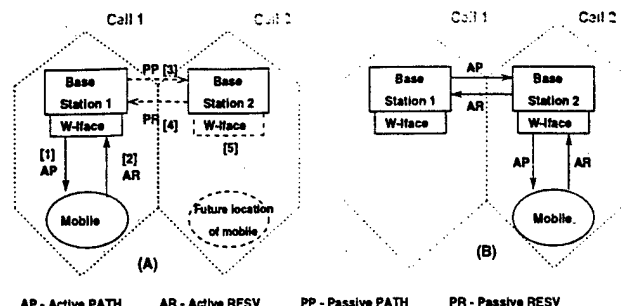
Figure 2: RSVP Messages for Reservation
