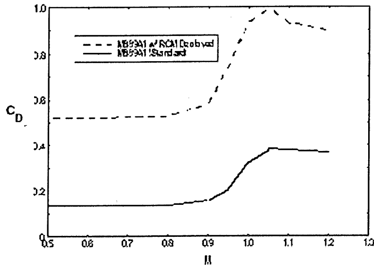
Figure 7. Drag Coefficient Versus Mach Number.
