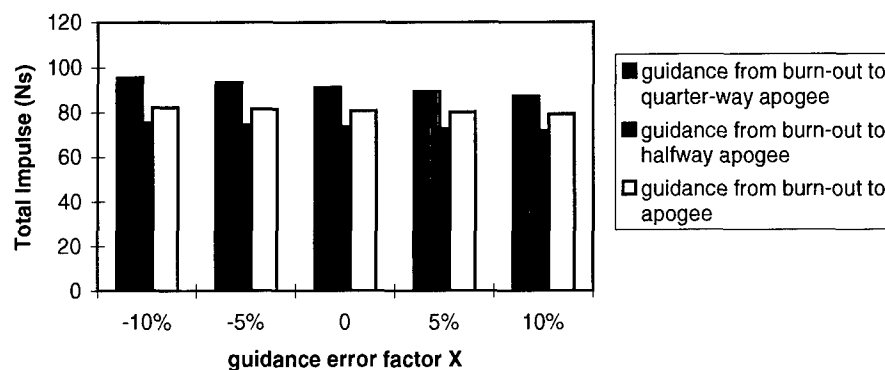
Figure 4.16: Required total side-thruster impulse for different guidance intervals and guidance error factors.
