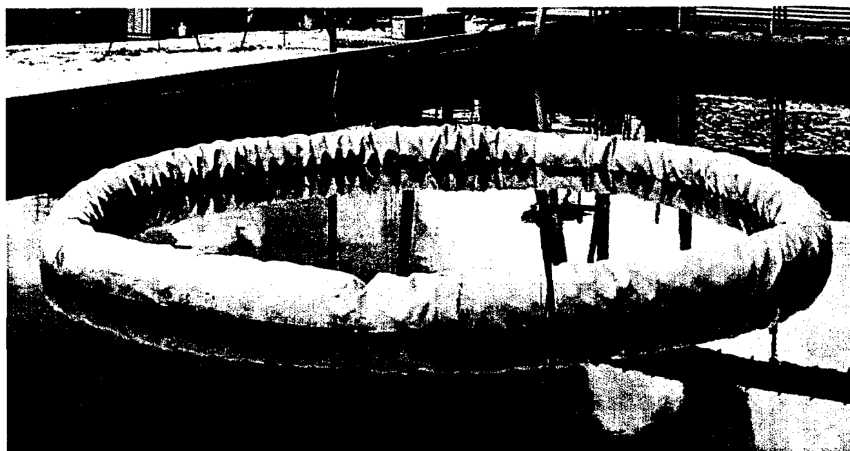
Figure F-2. Boom 6, before burning, in water.
