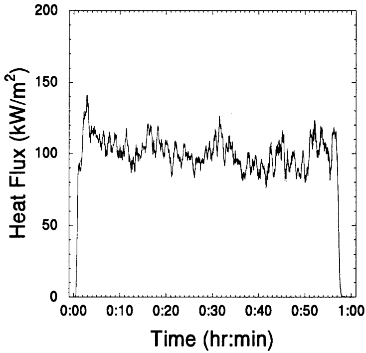
Figure G-12. Boom 5, Burn 4, vertical.
