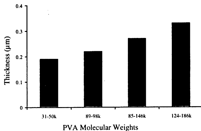
Figure 13. The influence of PVA molecular weights on the thickness of the cladding layer
