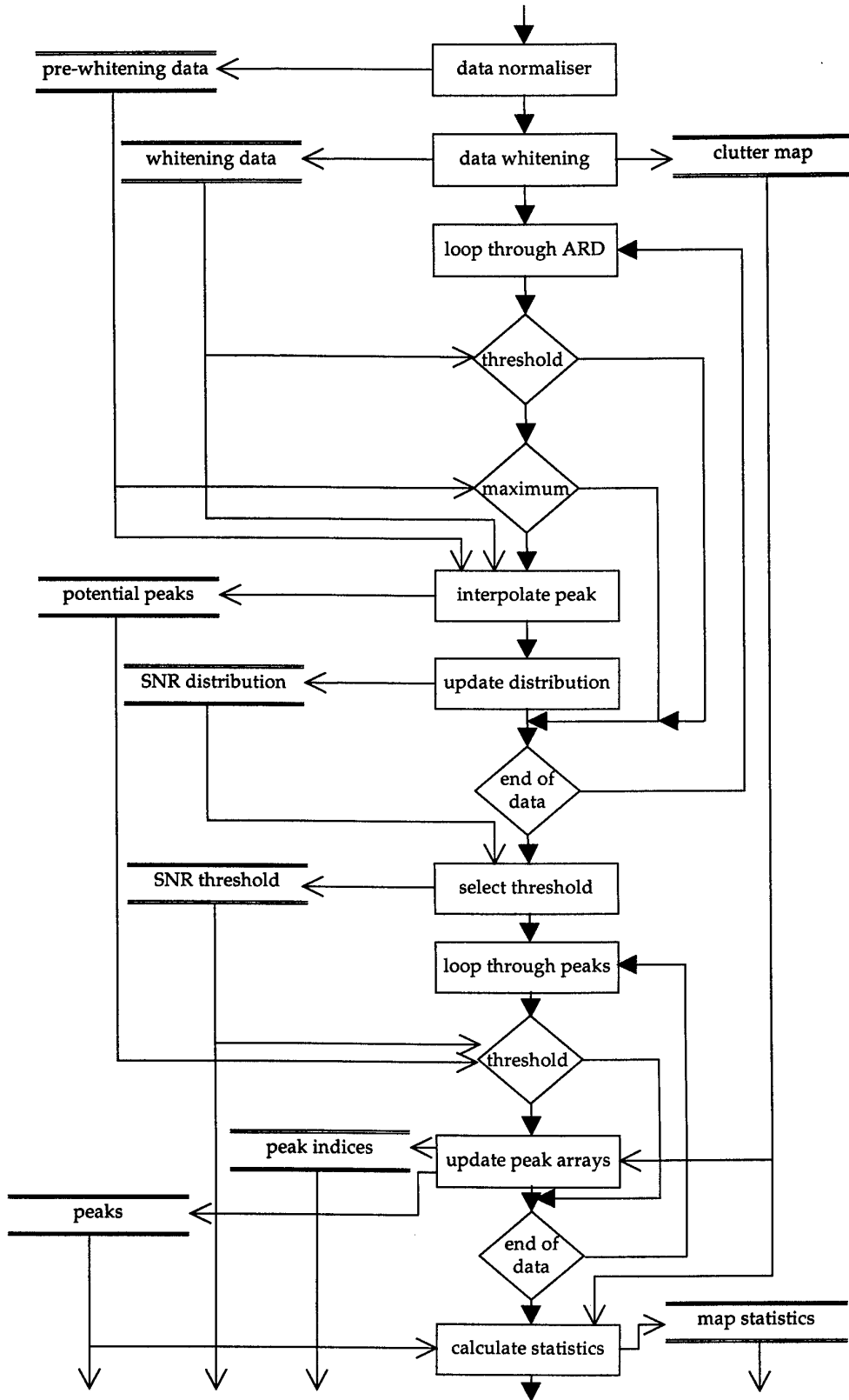
Figure 16 Modified peak detection flow diagram
