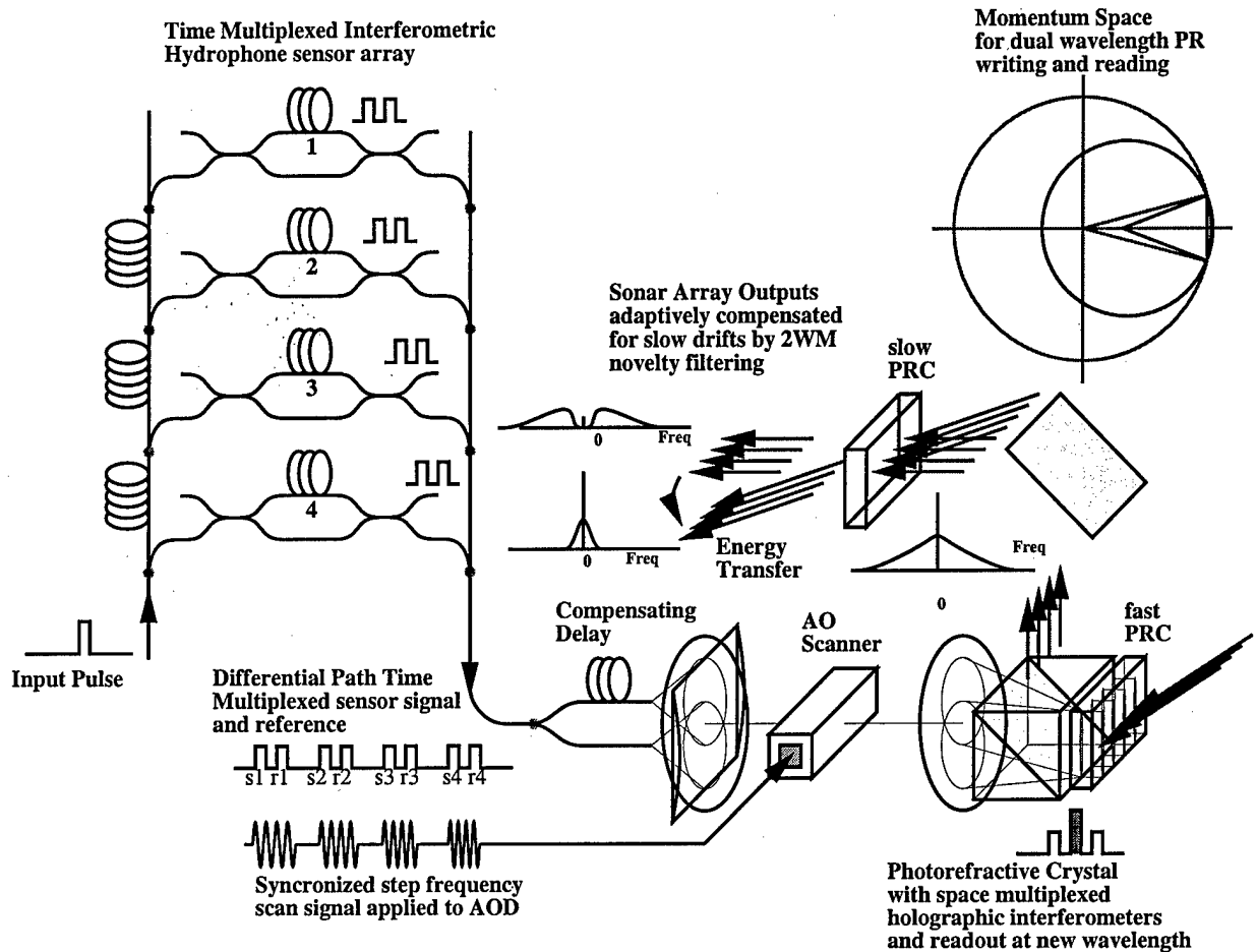
Figure 2: Sensor-Processor Interface: Optical preprocessing of the sonar signal to adaptively compensate for slow hydro-phone drift and novelty filtering of the optical carrier prior to beamforming.
