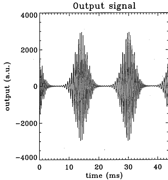
Figure 12: Cohered output from the array showing TTD processing achieving the full array gain on large fractional bandwidth signals
