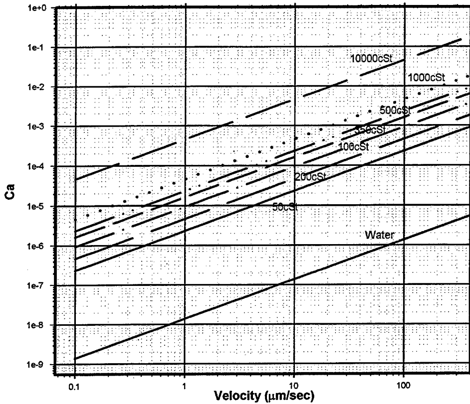
Figure 7. Capillary number vs. Velocity plot
