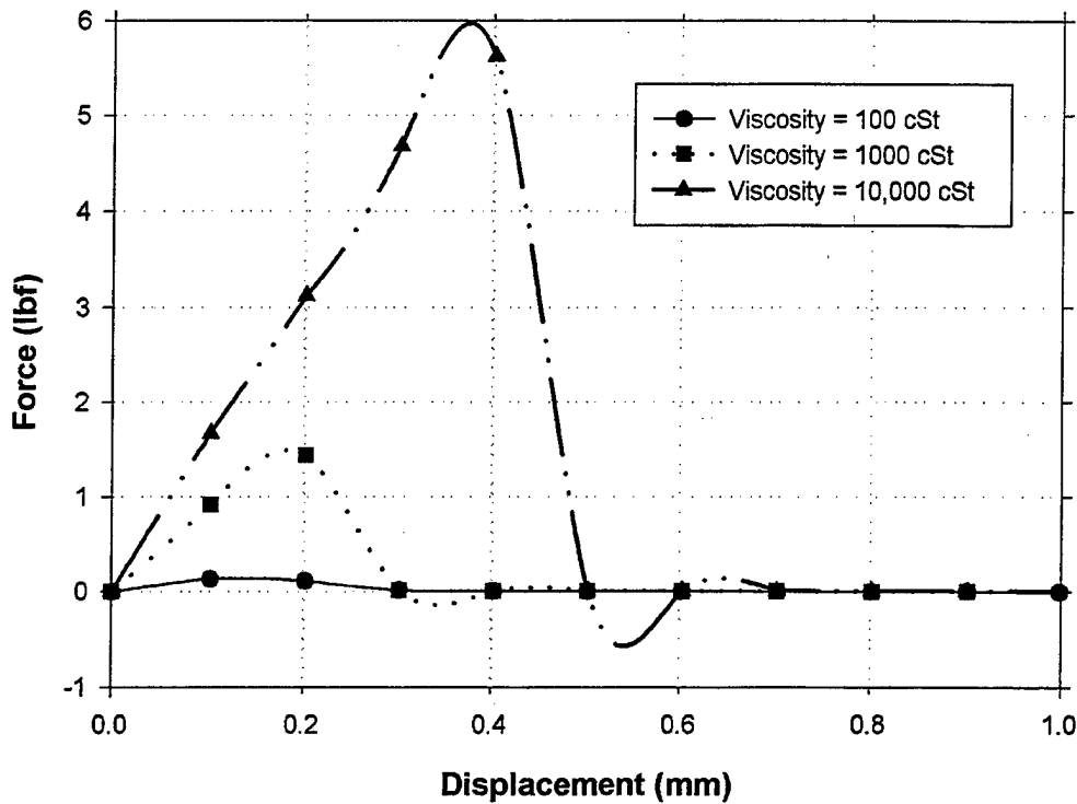
Figure 8. Force-Displacement plot that shows the effect of viscosity on F_{max} and d_{max} . Initial Liquid Layer Thickness ( l_0 ) is 200\mu\text{m} , and Separation Velocity ( V ) is 48\mu\text{m/s}
