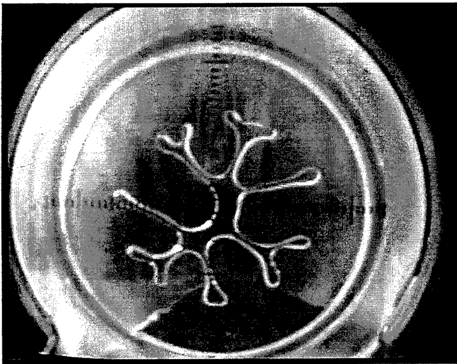
Figure 13d. Development of viscous fingering effect for 10,000 cSt Silicone Oil which has l_0 of 200 \mu m and Separation Velocity of 47 \mu m/s (Scale of 1 div=1mm)
