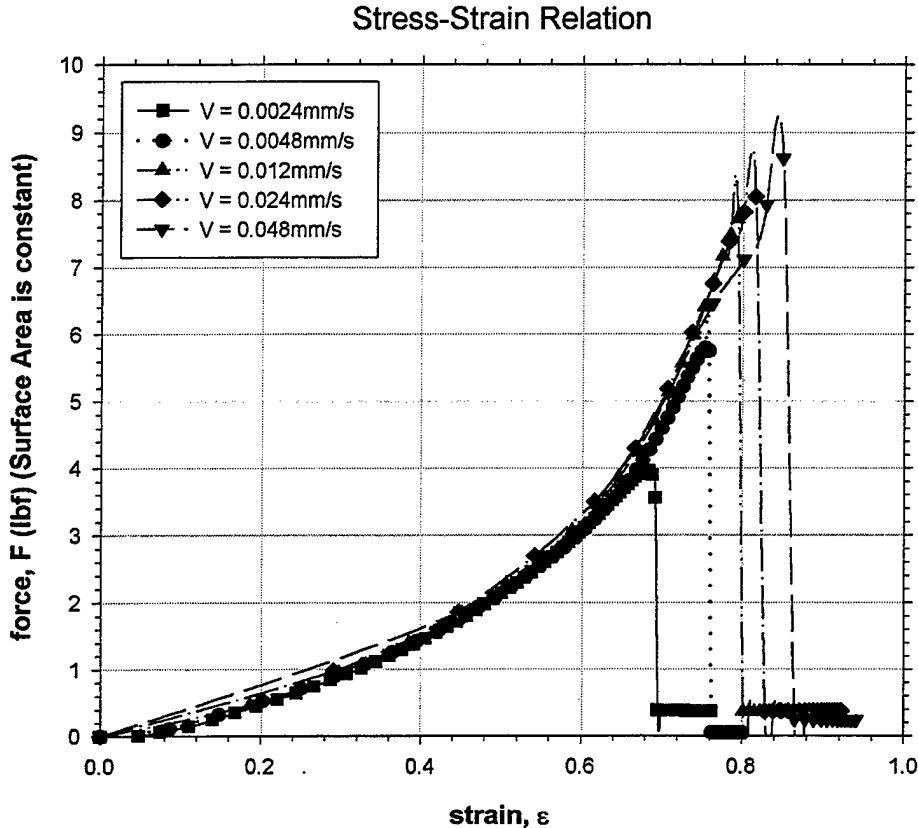
Figure 11. Stress-Strain plot for Initial Liquid Layer Thickness of 100 \mu m and liquid of 10,000 cSt Silicone Oil. For all curves surface area of the disk is constant ( A=\pi(2'')^2 )
