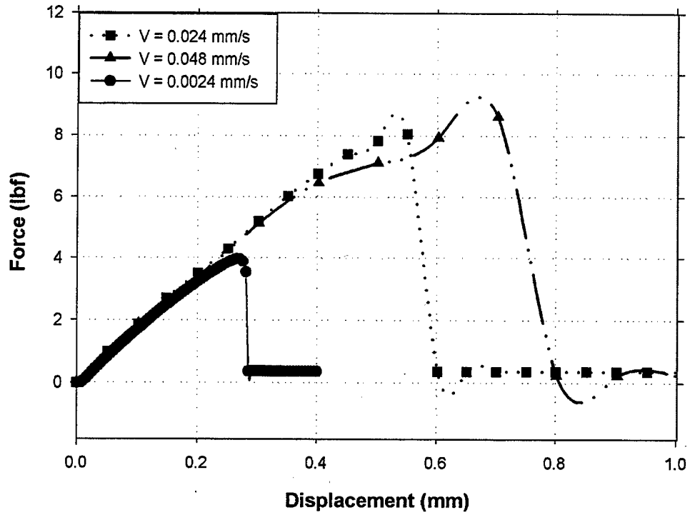
Figure 9. Force-Displacement plot that shows the effect of Separation Velocity on F_{max} and d_{max} . Initial Liquid Layer Thickness ( l_0 ) is 100\mu m
