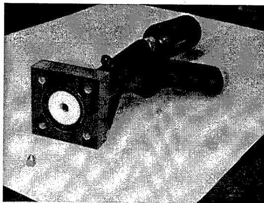
Figure 3.7 Paintball gun mechanism adapted for projectile injection.
