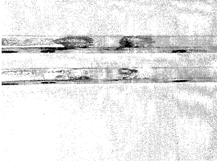
Figure 3.8 Rail damage due to arcing and plasma.
