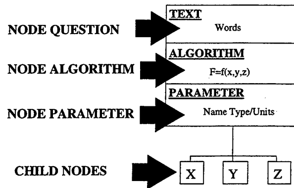
Figure 2. Node Characteristics
