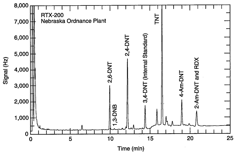
k) GC-ECD confirmation column (RTX-200), Nebraska Ordnance Plant.
