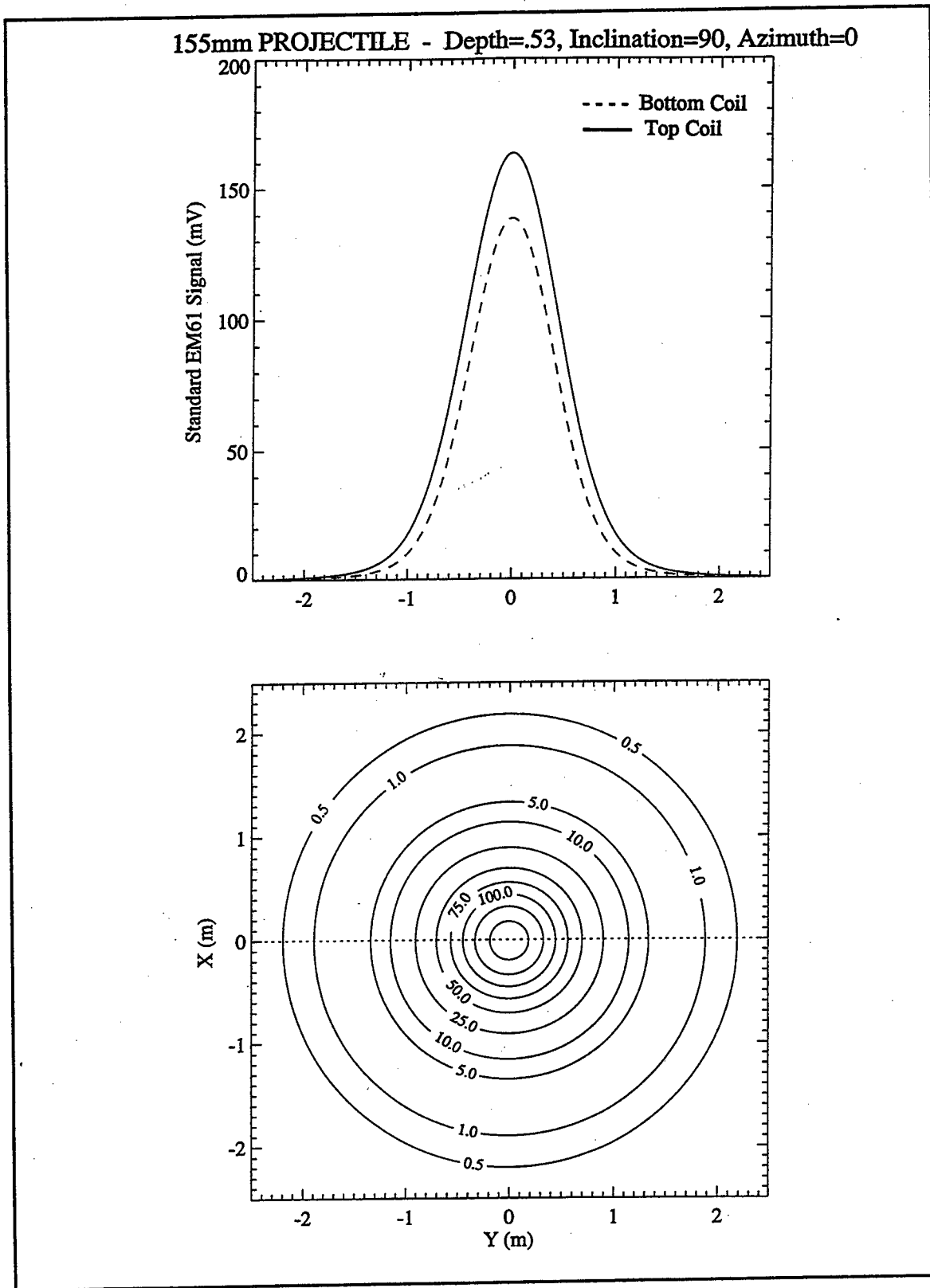
Figure 35. TDEM response calculation for a 155-mm projectile from the Phase III baseline; depth = 0.53 m, inclination = 90 deg, azimuth = 0 deg
