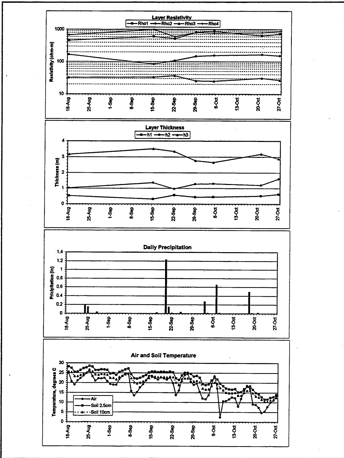
Figure 24. Electrical resistivity model parameters, precipitation, and air and soil temperatures as a function of date during the Phase IV demonstrations
