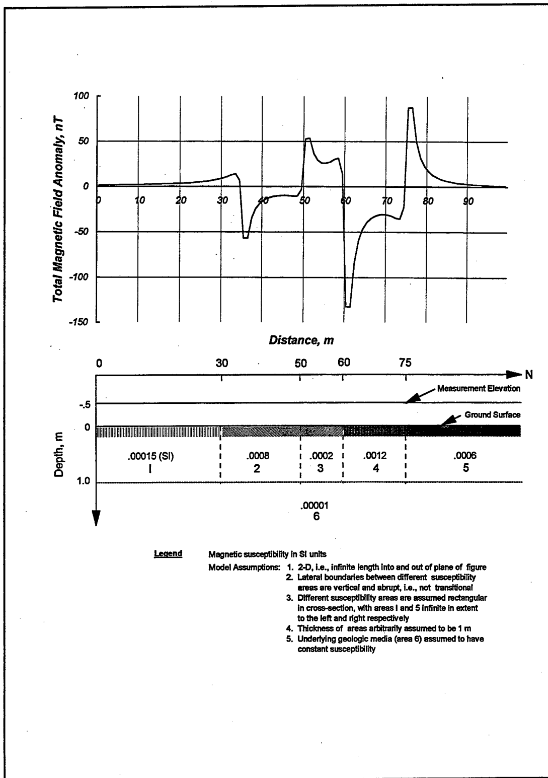
Figure 25. Total magnetic field anomaly calculations (2-D) for hypothetical model of susceptibility along line K based on Figure 21.
