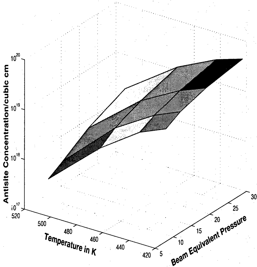
Figure 4.4: Model results of charged antisites concentration versus BEP and Temperature.
