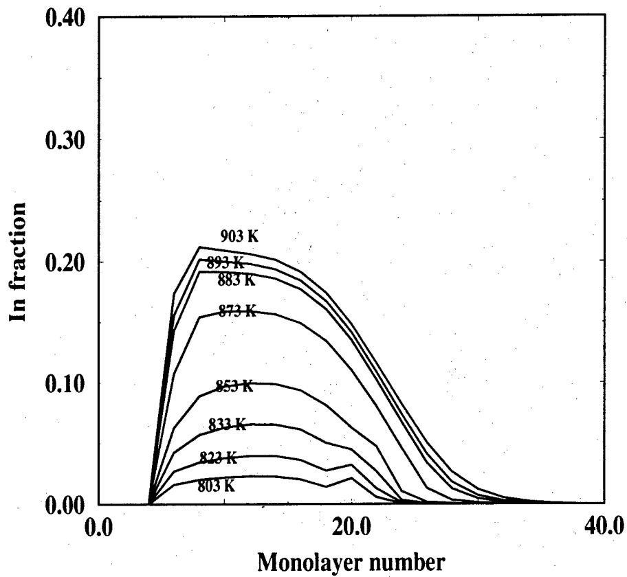
Figure 4.19: Simulation results of Indium composition versus monolayer number for various substrate temperatures for a As_4 BEP of 36 for 10 seconds growth.
