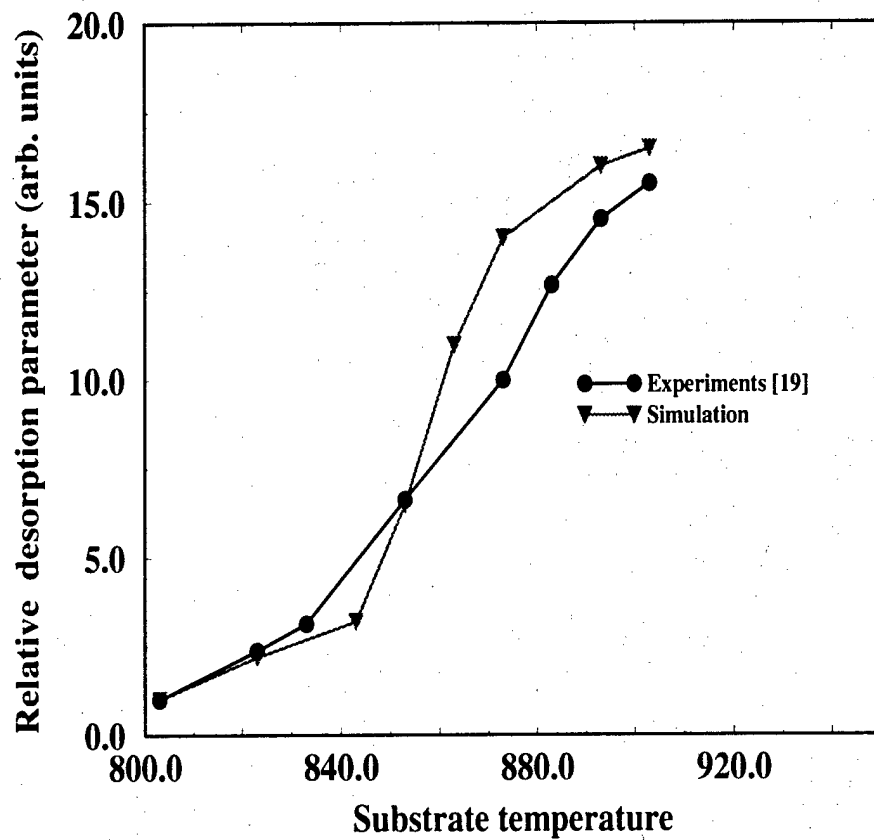
Figure 4.16: Comparison of simulation and experimental results [19] for relative desorption parameters of Indium versus substrate temperature for a As_4 BEP of 36 .
