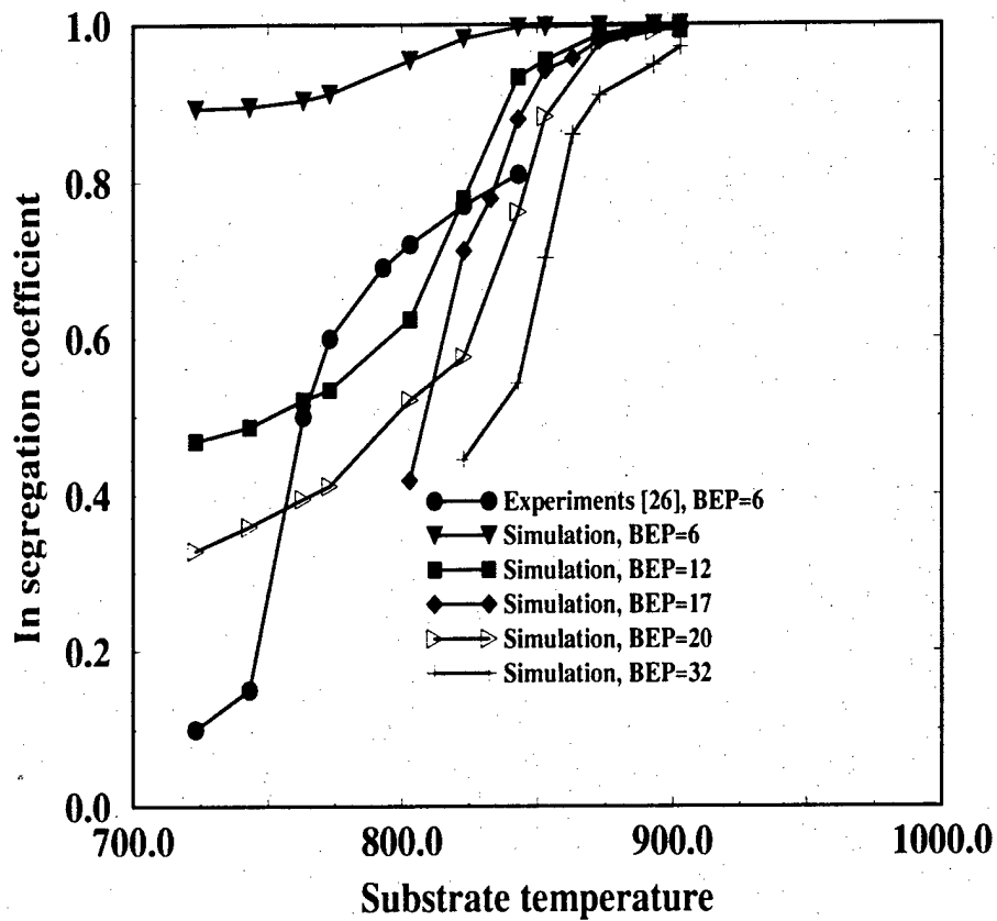
Figure 4.20: Simulation results of Indium segregation versus substrate temperatures for various As_4 and As_2 BEPs along with the experimental data of Kao et al [26] for a BEP of 6.
