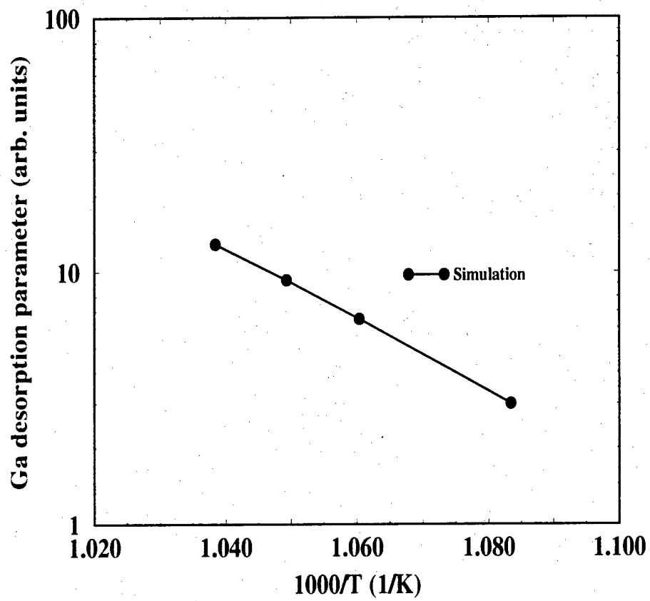
Figure 4.18: Simulation results of Ga desorption rate versus inverse of substrate temperature.
