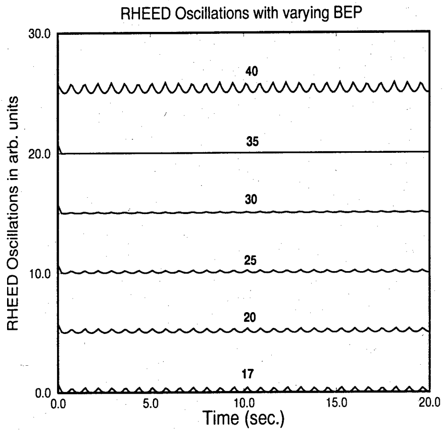
Figure 4.10: Model results of ROs versus time at 573°K for various BEP ratios at a growth rate of 1.4 \mu m/hr.
