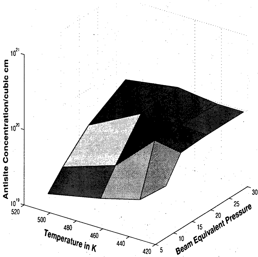
Figure 4.3: Model results of neutral antisites concentration versus BEP and Temperature.
