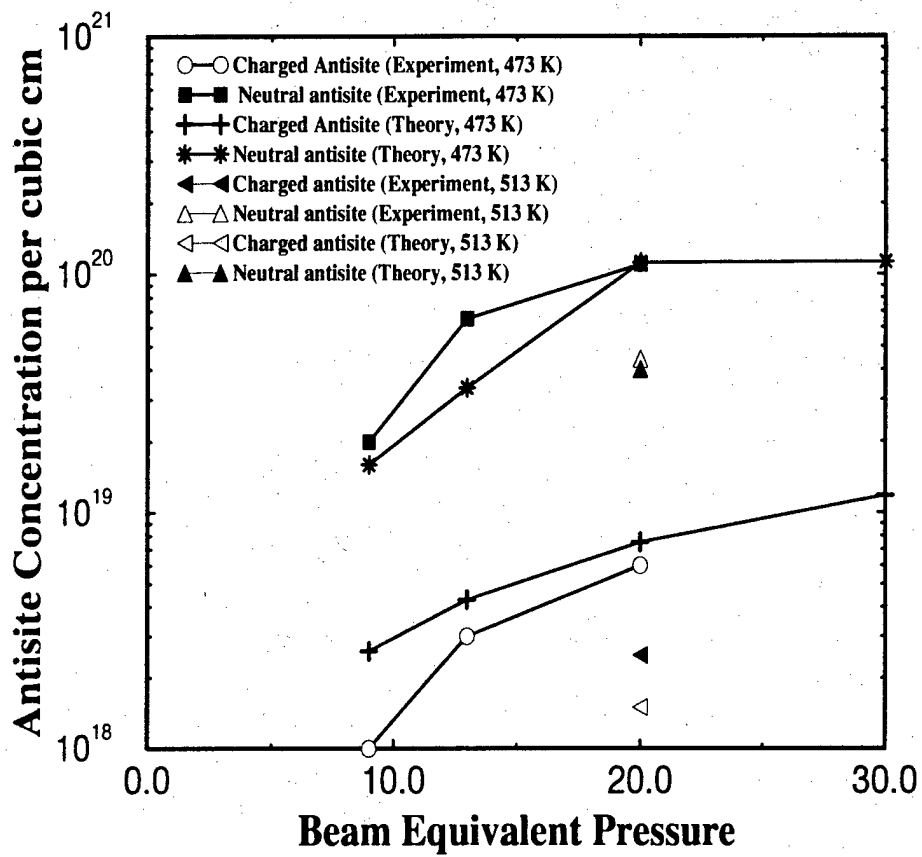
Figure 4.2: A plot of model results of charged and neutral antisite concentrations versus BEP along with the experimental results of Luysberg et al
