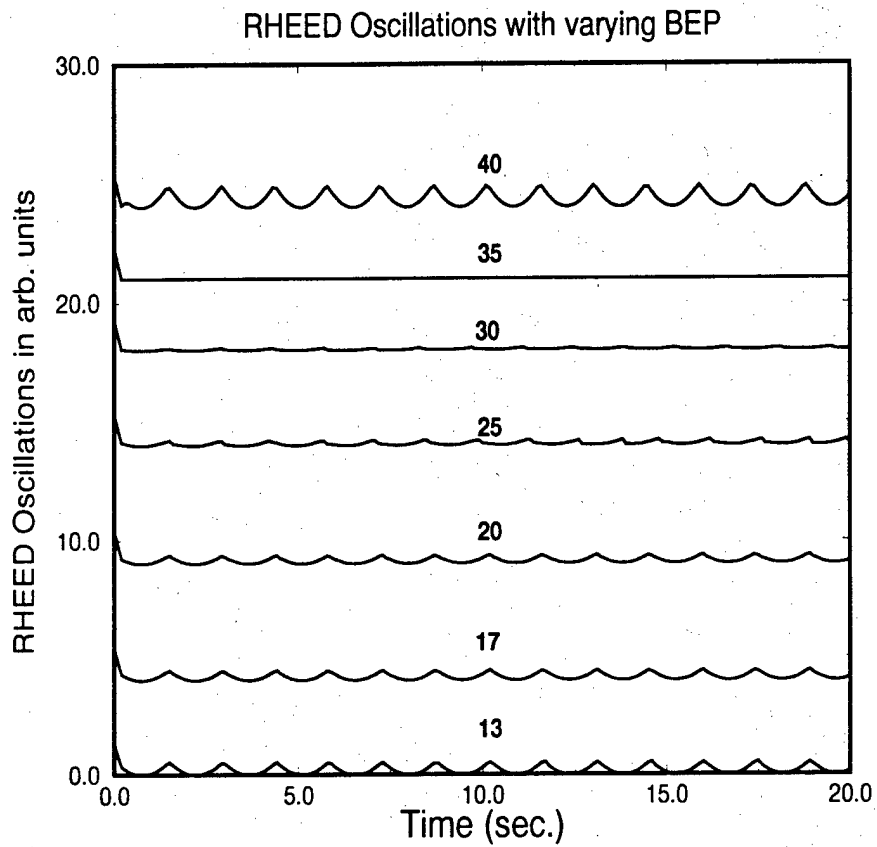
Figure 4.8: ROs versus time at 573°K for various BEP ratios at a growth rate of 0.7\mu\text{m/hr} . compared qualitatively with the experimental results of Shen et al : Fig. 1 of Ref.[18]
