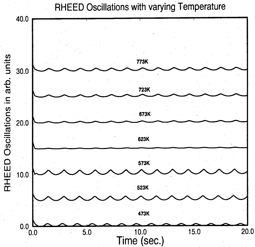
Figure 4.9: ROs versus time at 40 BEP for various temperatures at a growth rate of 0.7\mu\text{m/hr} . compared qualitatively with the experimental results of Shen et al : Fig. 3 of Ref. [18]
