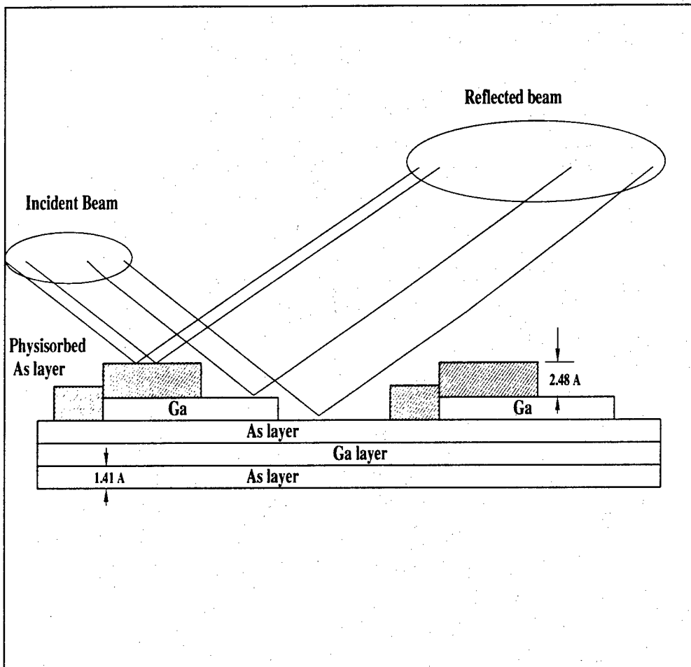
Figure 4.7: A schematic picture showing the reflected electron beams from the PA layer and the crystalline surface and the thicknesses of the layers.
