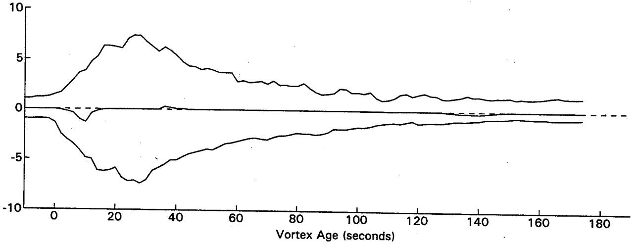
Maximum, Median, Minimum Crosswind (m/sec)
